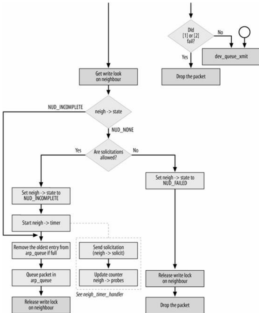
Figure 27-13b. ip_finish_output2 function: expanded version
