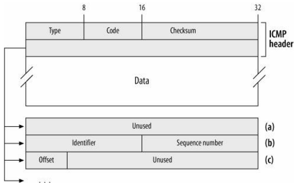
Figure 25-1. ICMP header
