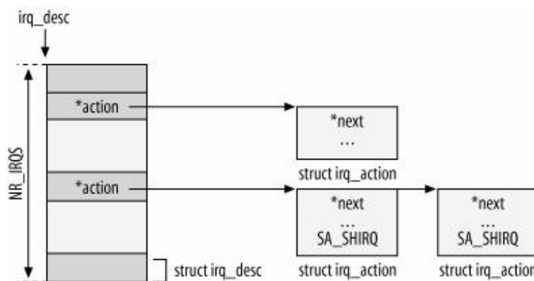
Figure 5-2. Organization of IRQ handlers
