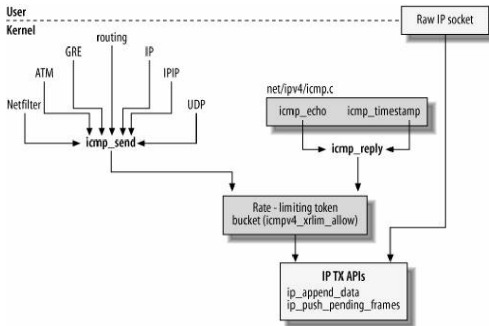
Figure 25-8. Subsystems using icmp_send/icmp_reply
