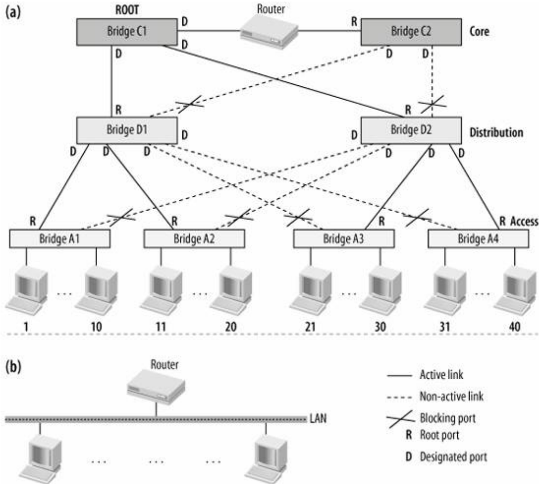
Figure 15-2. Hierarchical bridged L2 topology
