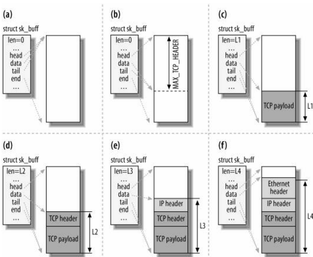
Figure 2-8. Buffer that is filled in while traversing the stack from the TCP layer down to the link layer
