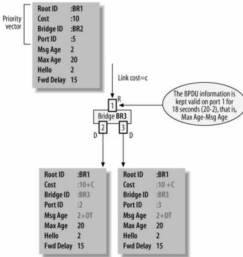
Figure 15-9. BPDU relaying via nonroot bridges
