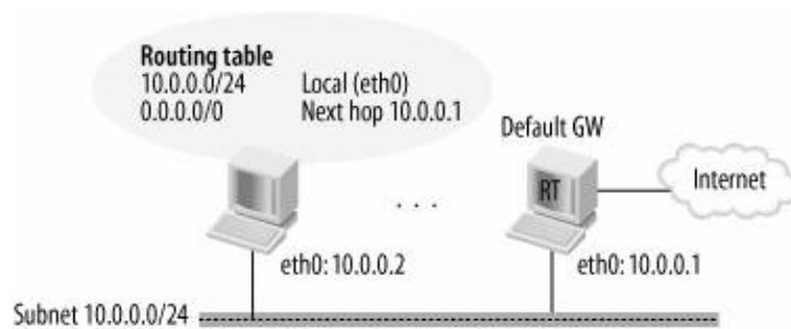
Figure 30-2. Basic example of router and routing table
