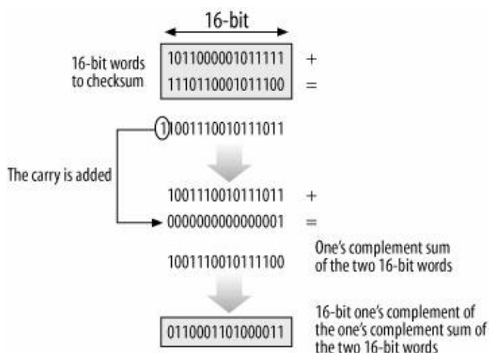
Figure 18-13. IP checksum computation
