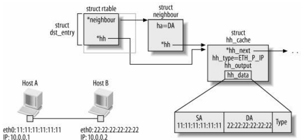
Figure 27-1. Relationship among dst_entry , neighbour , and hh_cache structures
