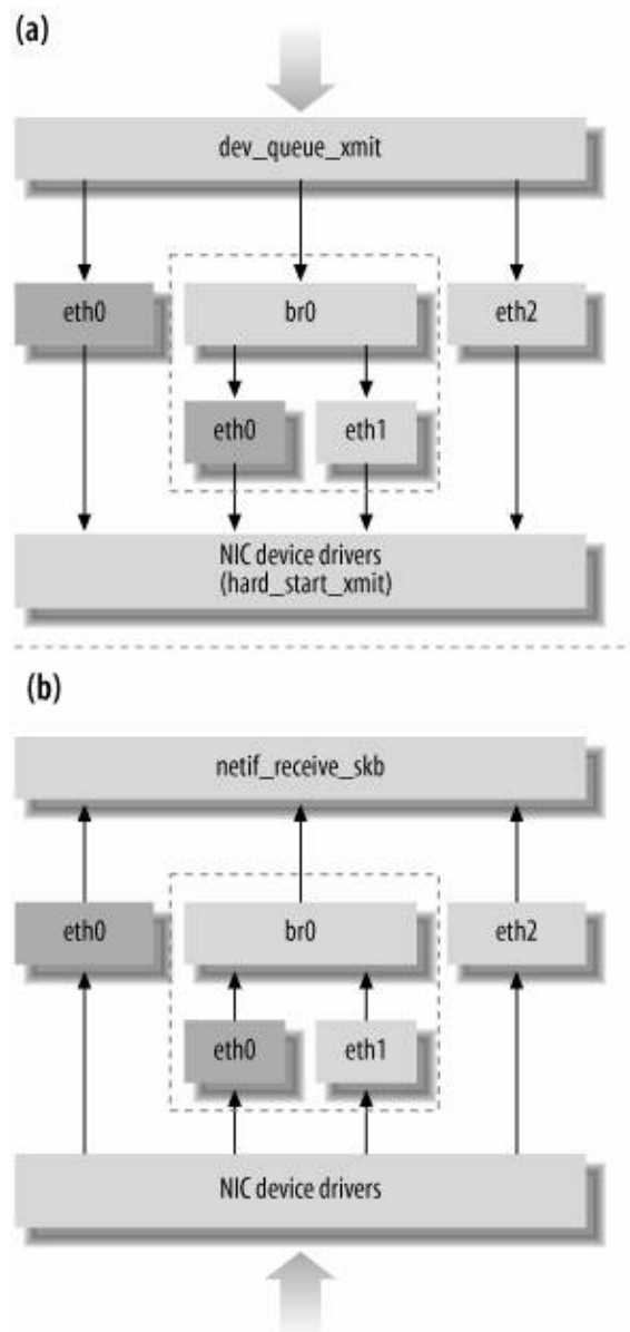
Figure 16-5. Using a NIC both as a standalone interface and as a bridge port
