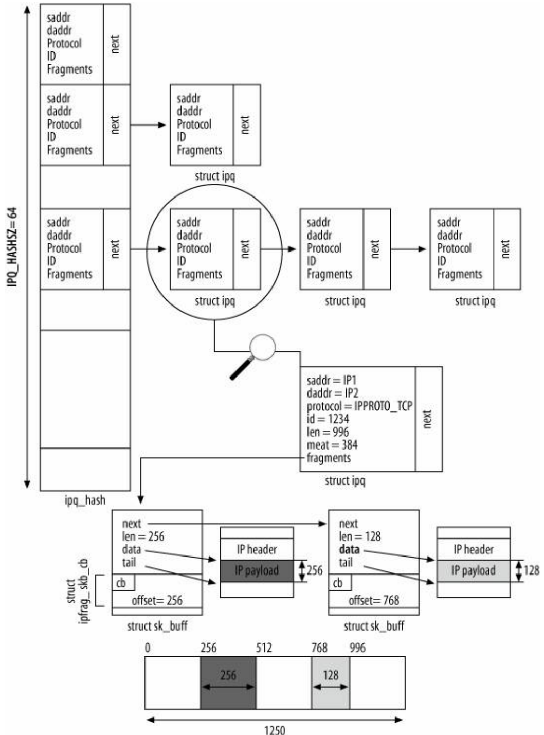
Figure 22-1. Structure used to store IP fragments
