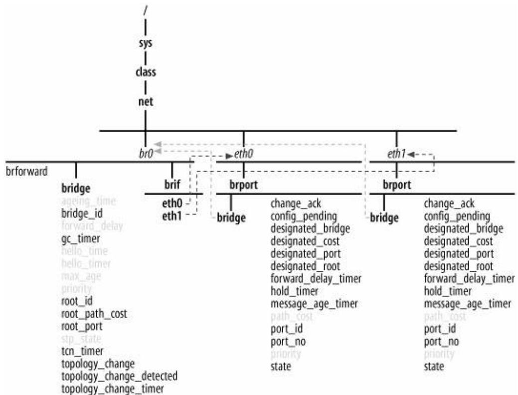
Figure 17-2. Example of bridge information exported with sysfs
