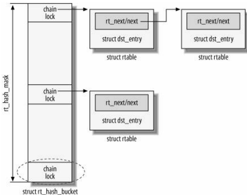
Figure 33-1. Routing cache structure
