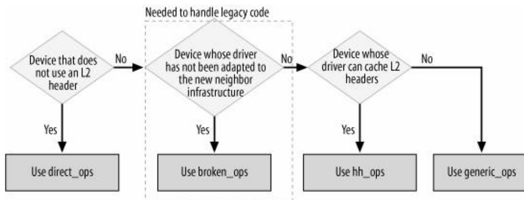
Figure 28-12. Initialization of neigh->ops in arp_constructor
