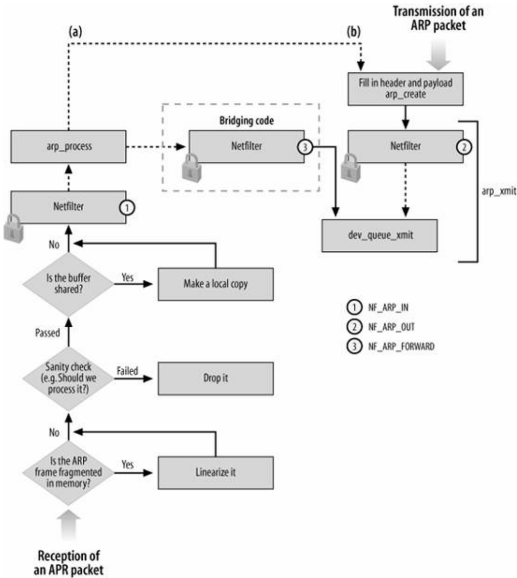
Figure 28-13. (a) arp_rcv; (b) arp_send
