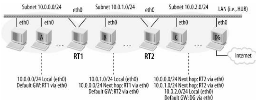
Figure 31-10. Sample configuration for a shared media topology
