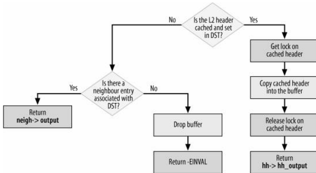
Figure 27-12. ip_finish_output2 function: compact version
