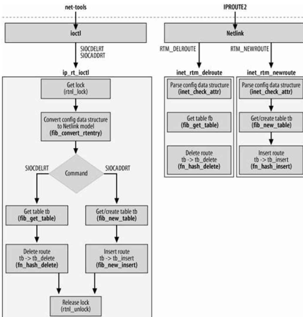
Figure 36-1. ioctl -based versus Netlink-based routing table manipulation
