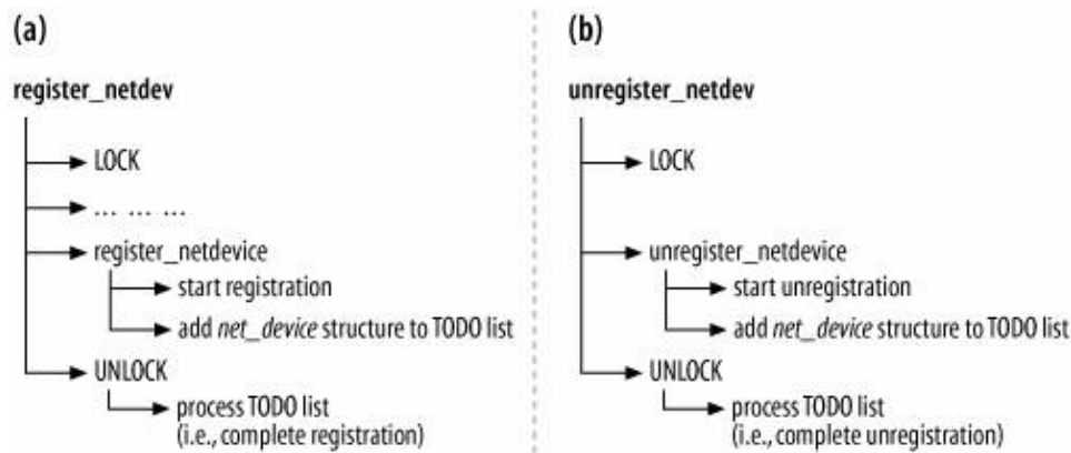
Figure 8-5. Structure of register_netdev and unregister_netdev
