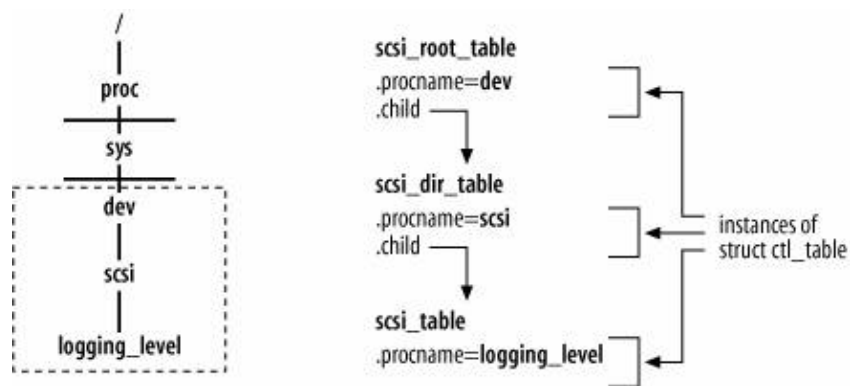
Figure 3-1. Registration of the /proc/sys/dev/scsi/logging_level file
