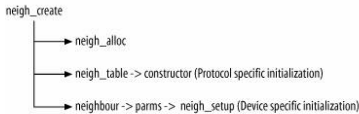
Figure 28-11. Initialization sequence for a new neighbour structure
