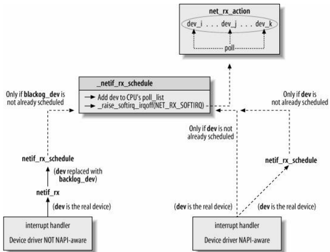
Figure 10-2. NAPI-aware drivers versus non-NAPI-aware devices
