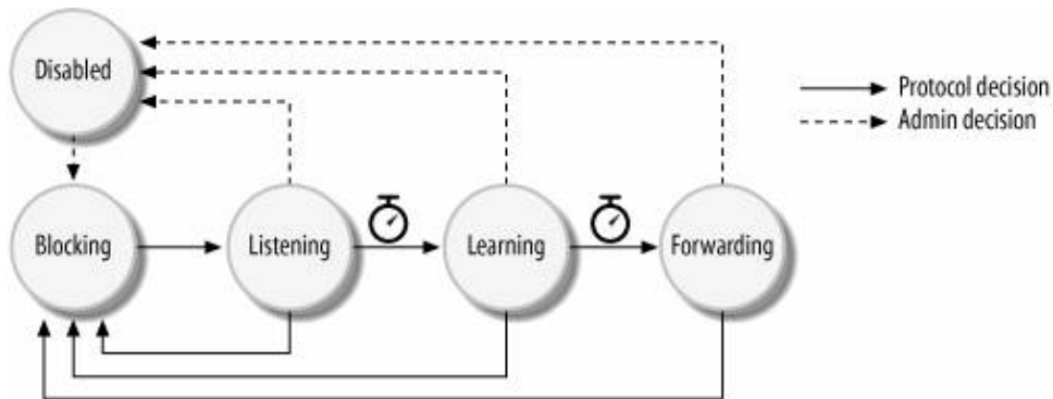
Figure 15-6. Port state transitions
