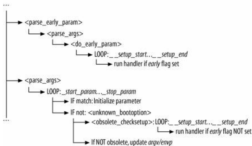
Figure 7-2. Two-pass option parsing
