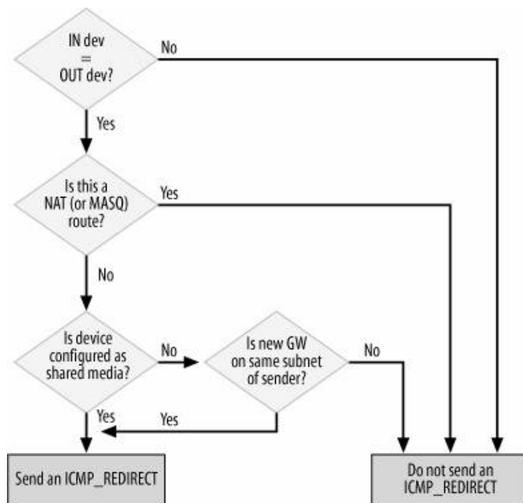
Figure 31-11. Conditions needed to generate an ICMP REDIRECT
