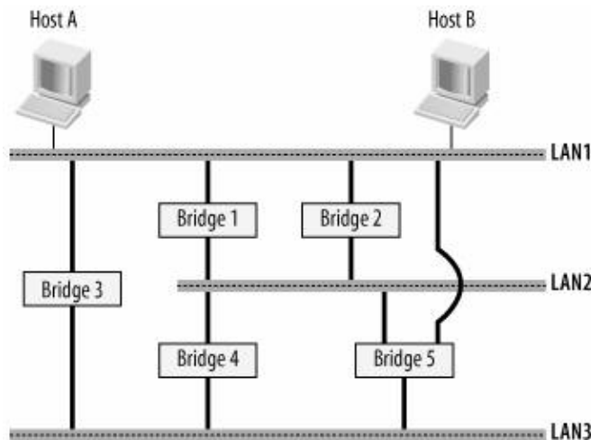
Figure 14-9. Topology with multiple loops
