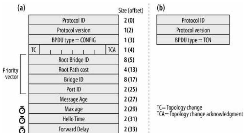
Figure 15-8. a) Configuration BPDU; b) BPDU
