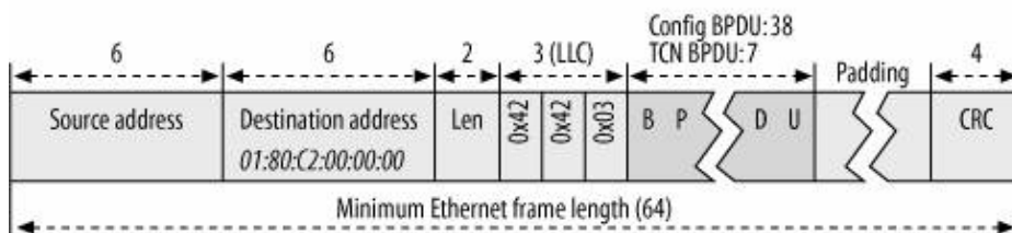
Figure 15-20. BPDU encapsulation
