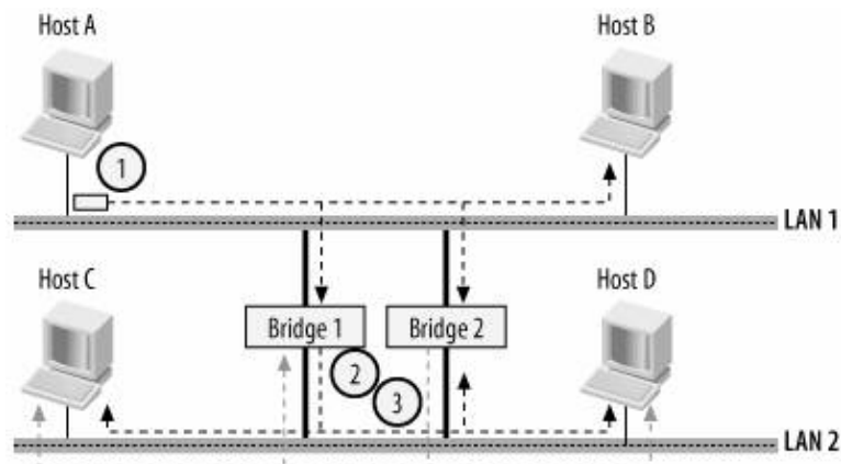
Figure 14-8. Bridging loop
