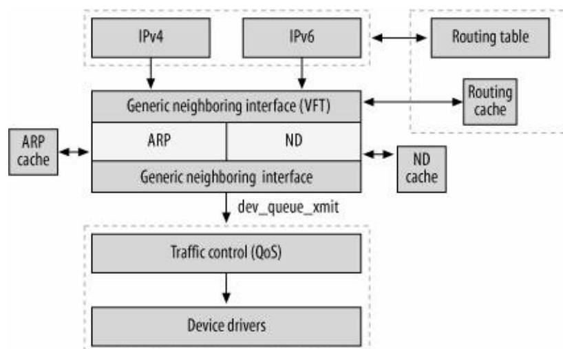
Figure 26-5. The big picture
