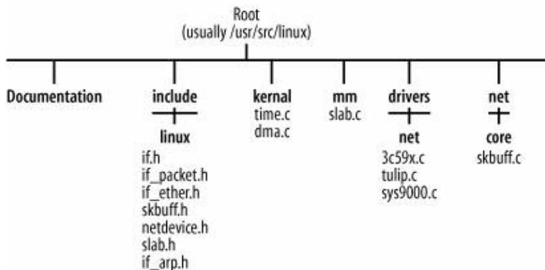
Figure 2-11. Files referenced in this chapter
