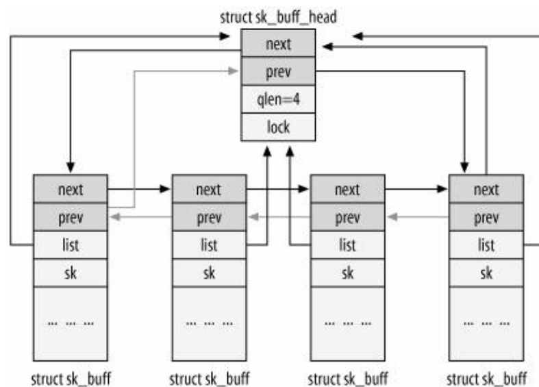
Figure 2-1. List of sk_buff elements
