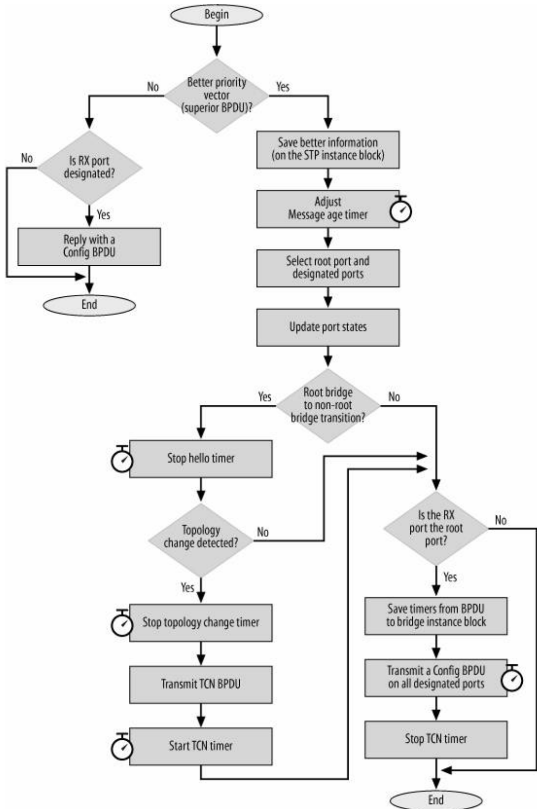
Figure 15-22. Processing ingress configuration BPDUs
