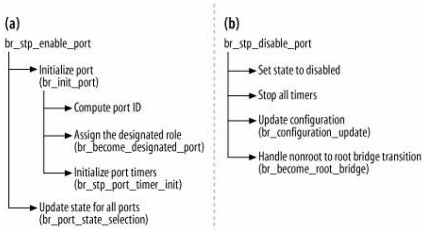
Figure 16-10. (a) Enabling a port; (b) disabling a port
