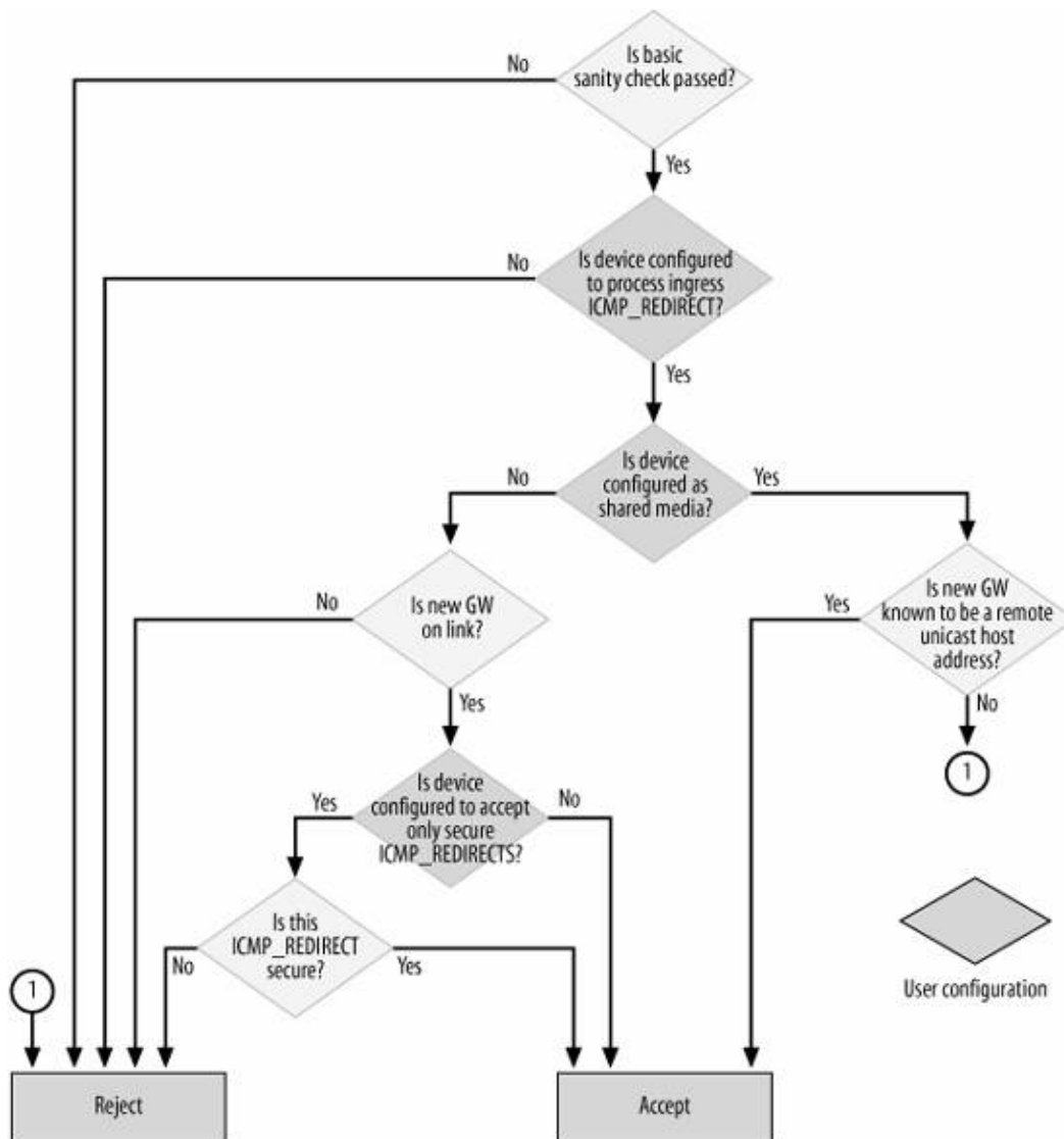
Figure 31-12. Conditions needed to process an ingress ICMP REDIRECT
