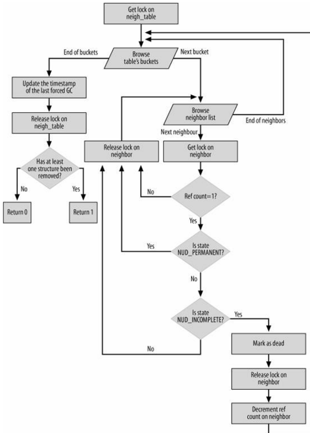
Figure 27-7. neigh_forced_gc function
