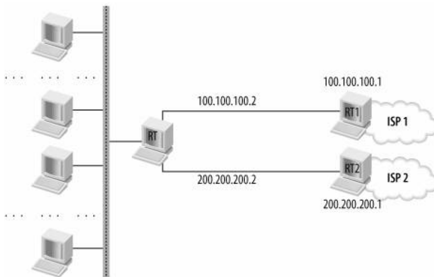
Figure 31-3. Example of topology with multipath
