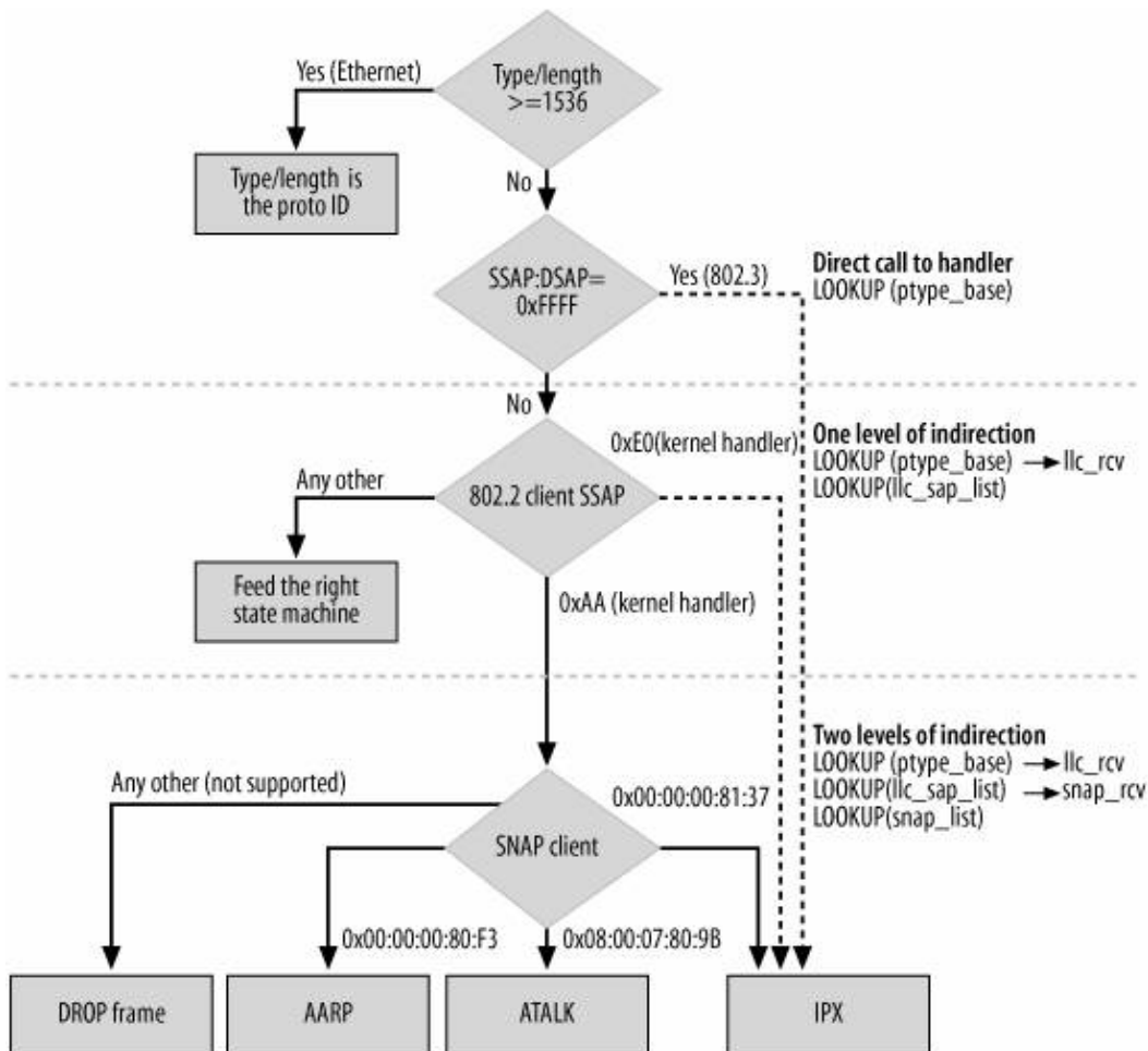
Figure 13-11. Protocol detection for Ethernet/802.3/802.2/SNAP frames
