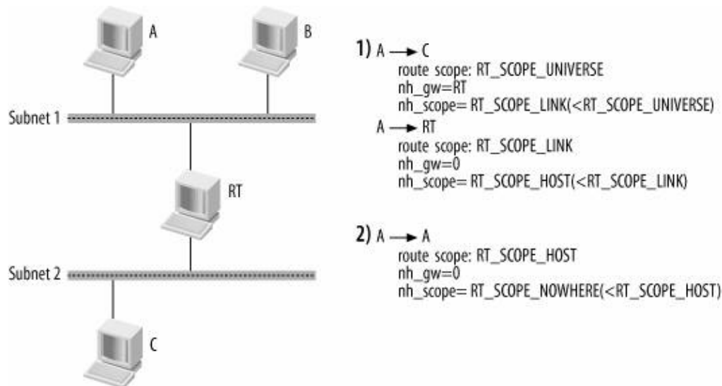
Figure 32-3. Example of initialization of next hop's scopes
