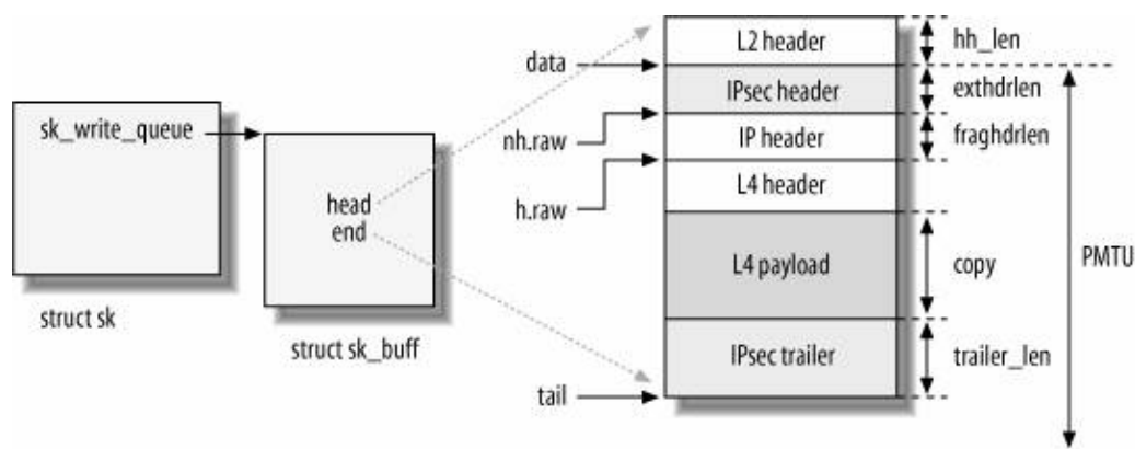
Figure 21-2. IP packet that does not need fragmentation, with IPsec
