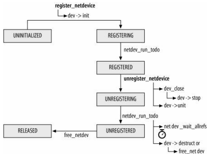
Figure 8-4. net_device's registration state machine
