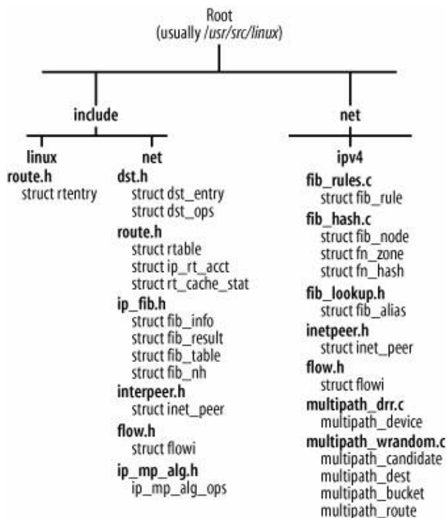
Figure 36-5. Distribution of data structures in kernel files
