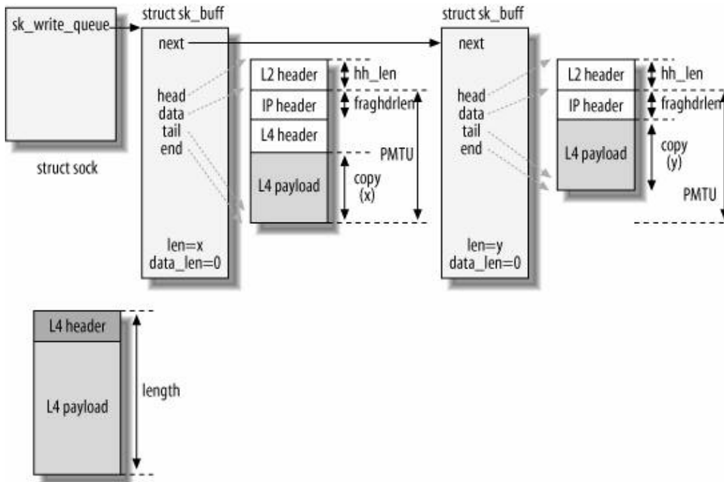
Figure 21-3. Fragmentation without Scatter/Gather I/O, no MSG_MORE
