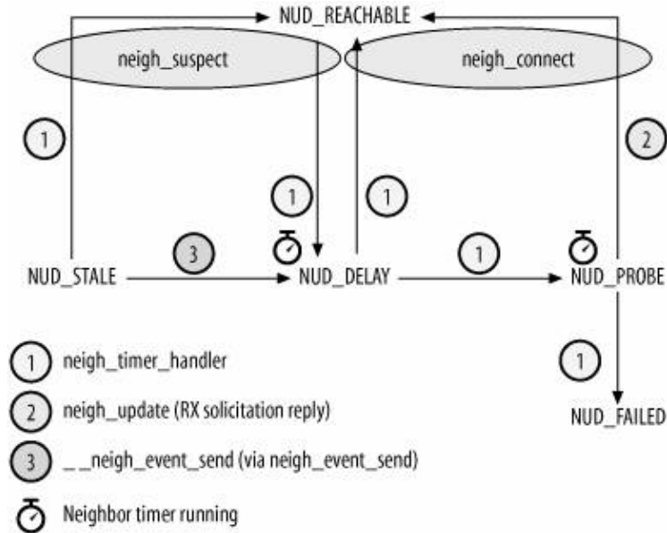
Figure 27-4. Possible state transitions for a neighbor that has been resolved at least once
