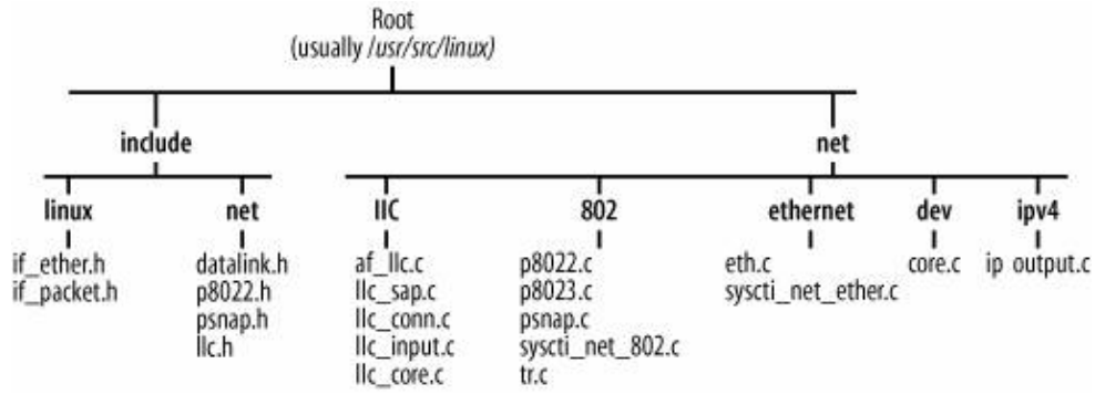
Figure 13-12. Files and directories featured in this chapter
