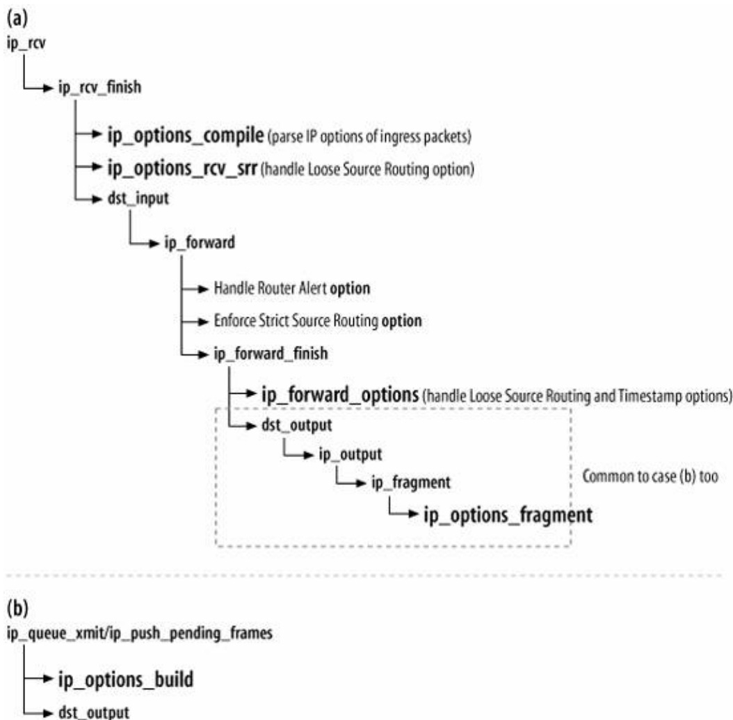
Figure 19-3. (a) Ingress packets; (b) locally generated packets
