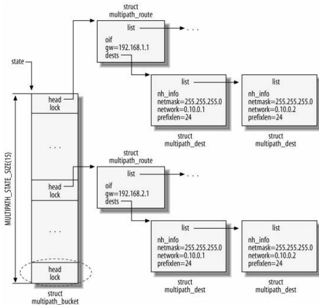
Figure 33-4. Next-hop database created by the weighted random algorithm
