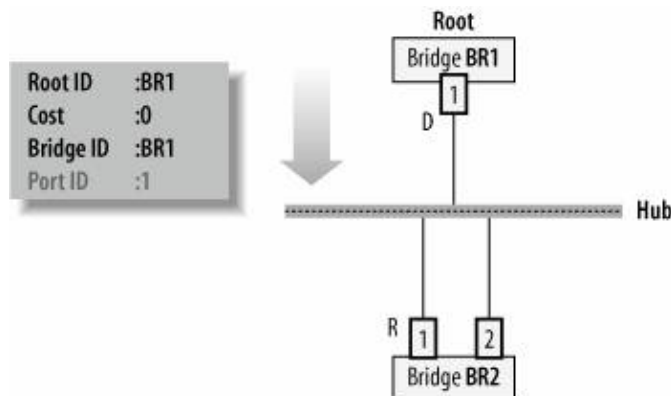
Figure 15-10. Multiple candidates for the root port selection
