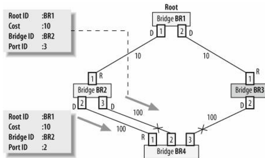
Figure 15-14. Port ID as the tiebreaker
