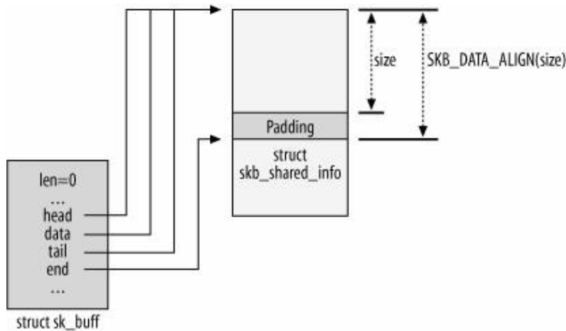
Figure 2-5. alloc_skb function
