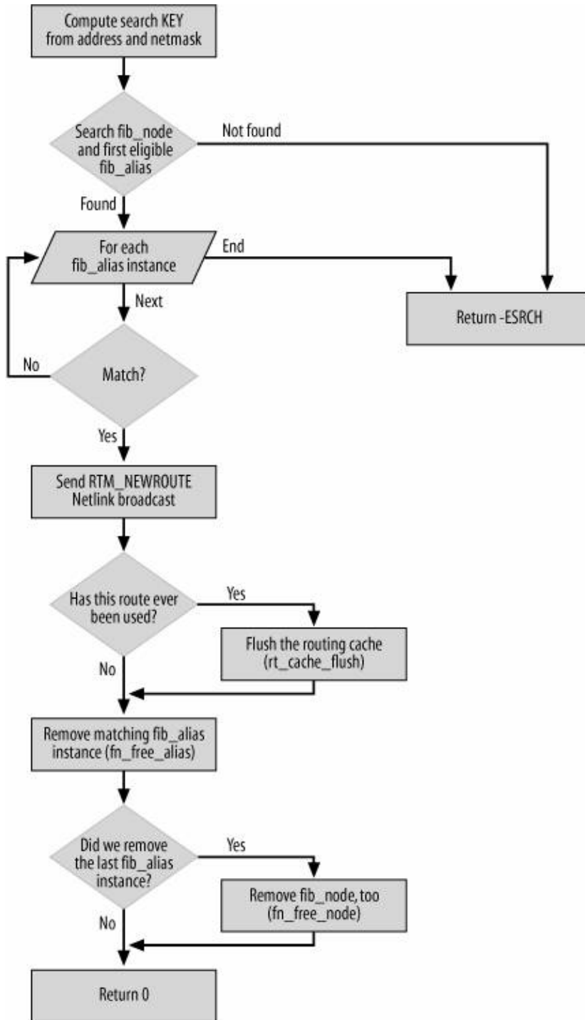
Figure 34-4. fn_hash_delete function
