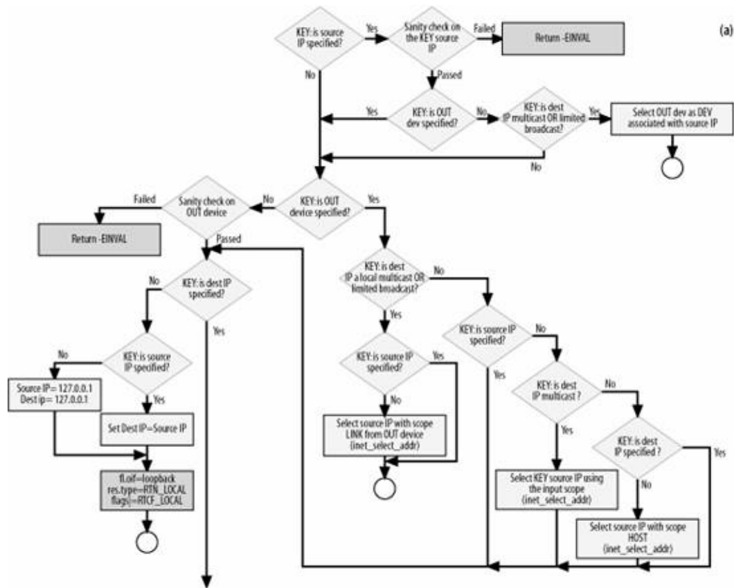
Figure 35-8a. ip_route_output_slow function
