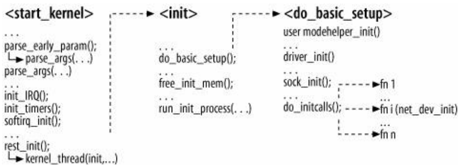
Figure 5-1. Kernel initialization
