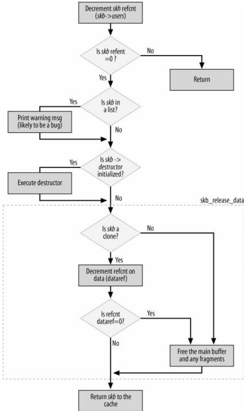
Figure 2-6. kfree_skb function
