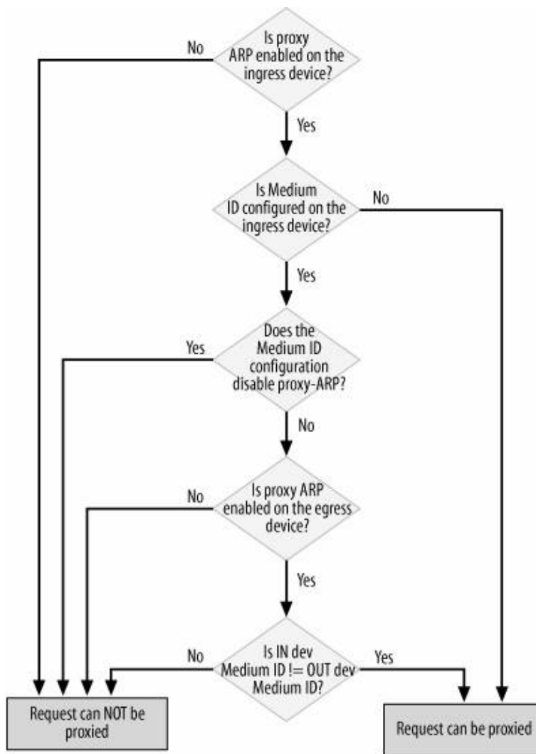
Figure 28-10. arp_fwd_proxy function
