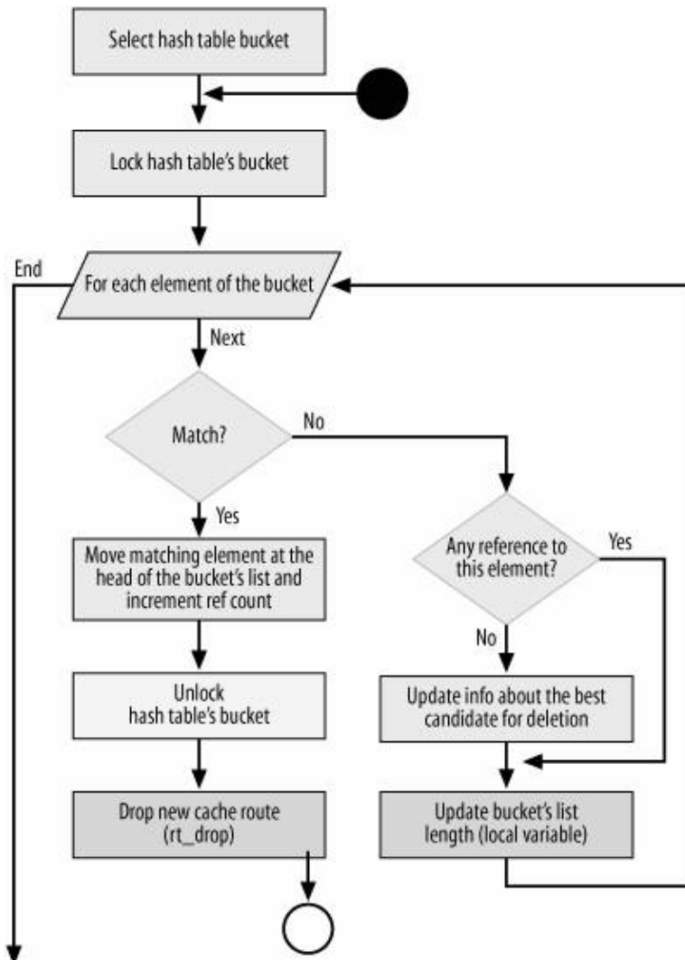
Figure 33-2a. rt_intern_hash function
