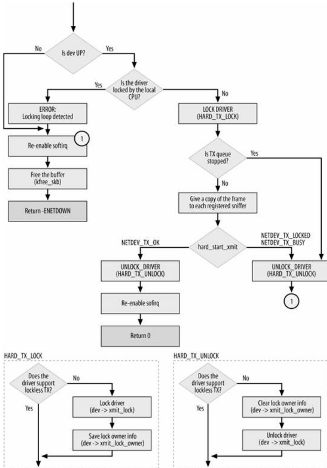
Figure 11-3b. dev_queue_xmit function
