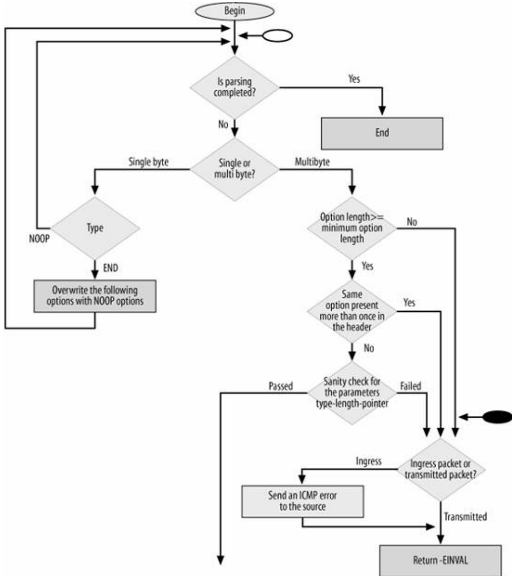
Figure 19-5a. ip_options_compile overview
