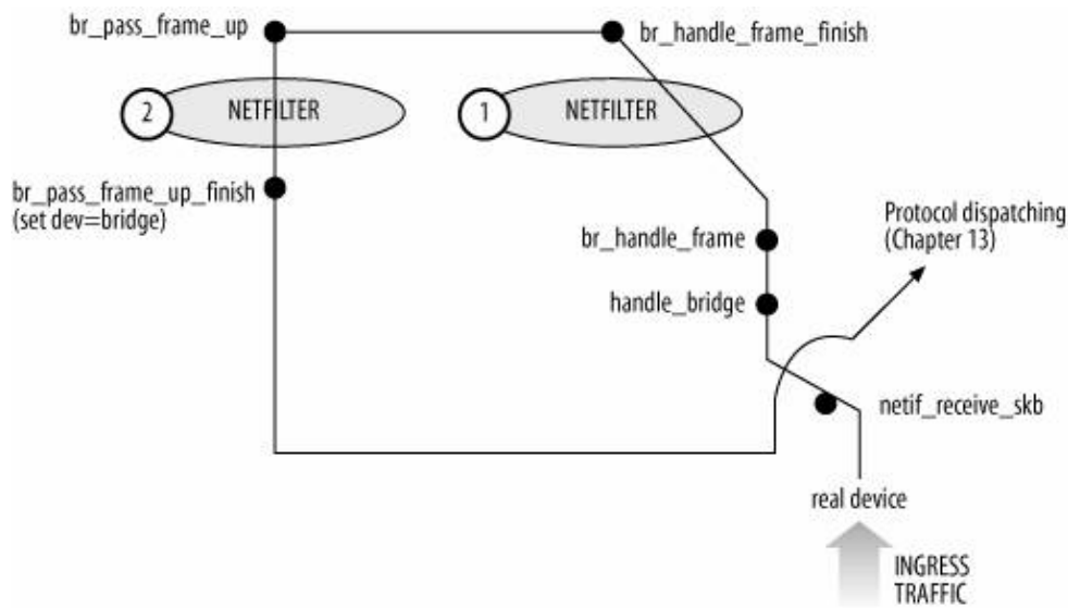
Figure 16-14. Local delivery of ingress data frames
