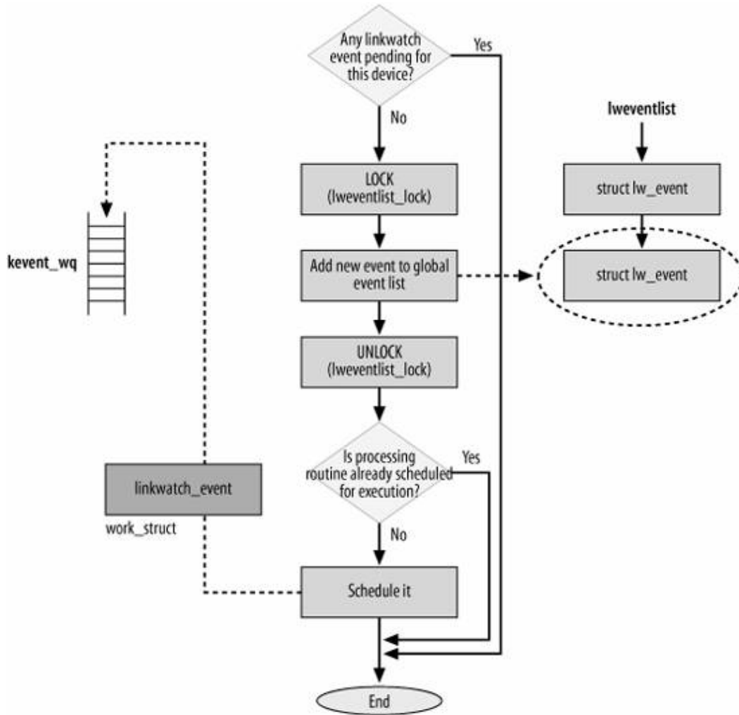
Figure 8-7. linkwatch_fire_event function
