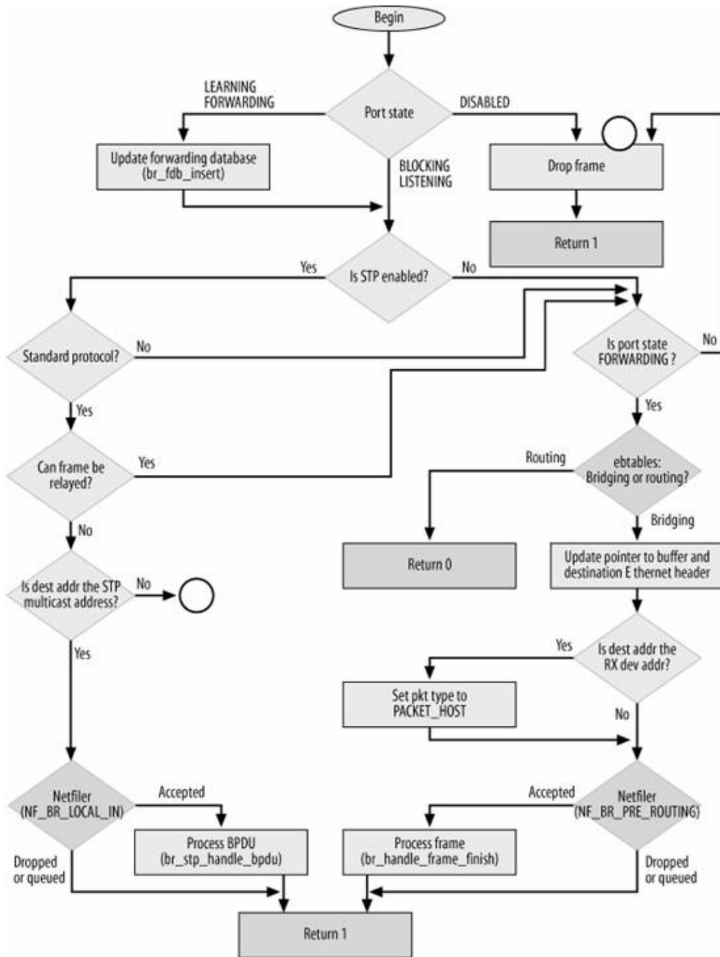
Figure 16-12. br_handle_frame function
