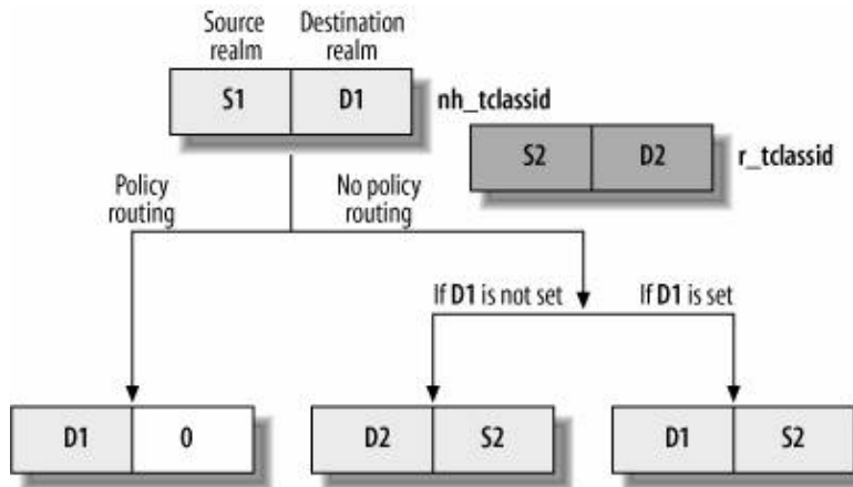
Figure 35-19. fib_combine_itag function
