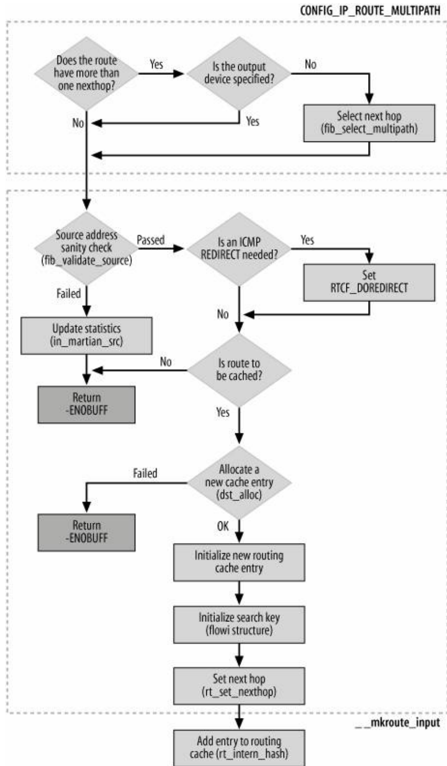
Figure 35-7. ip_mkroute_input function
