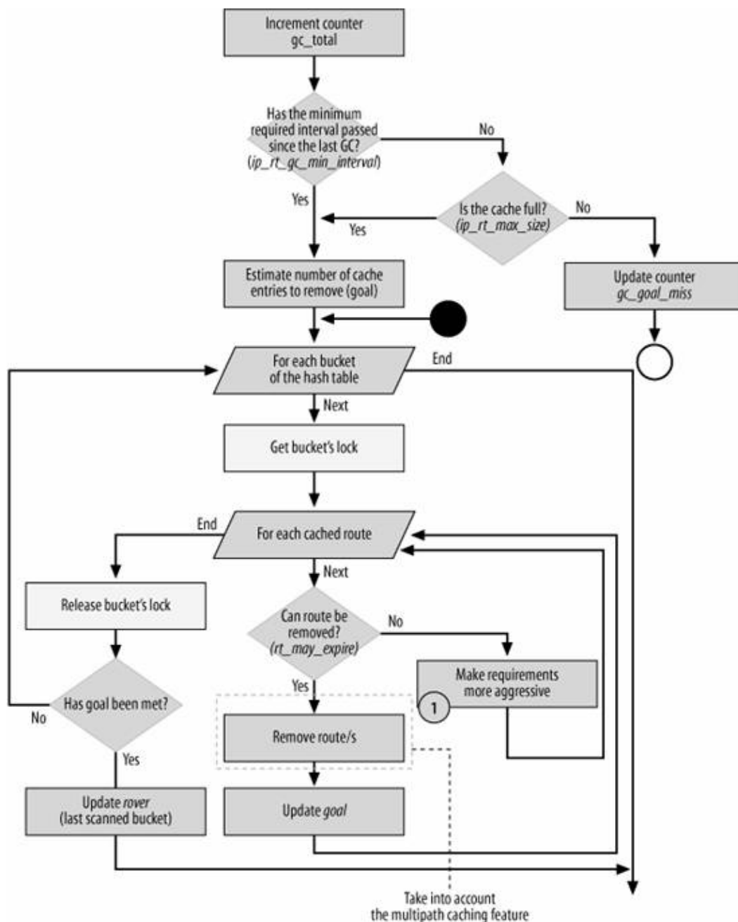
Figure 33-8a. rt_garbage_collect function
