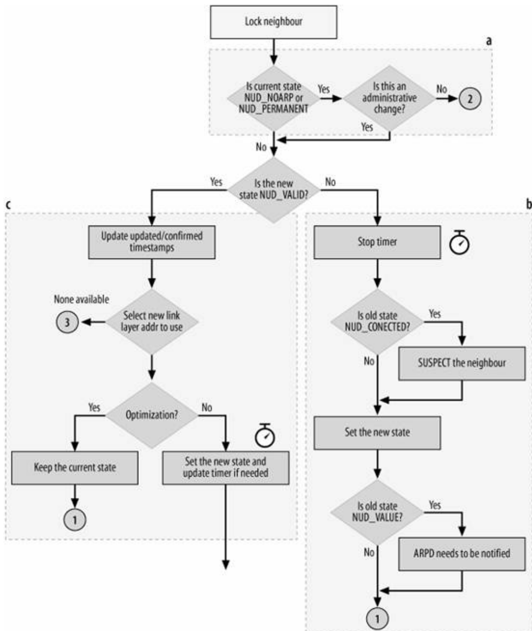
Figure 27-5a. neigh_update function
