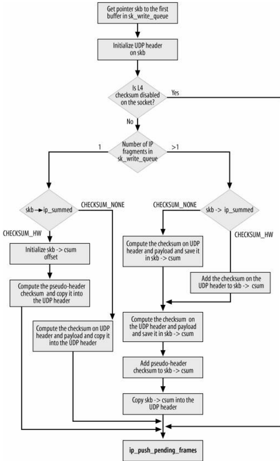
Figure 21-13. udp_push_pending_frames function
