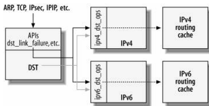
Figure 33-6. dst_ops interface
