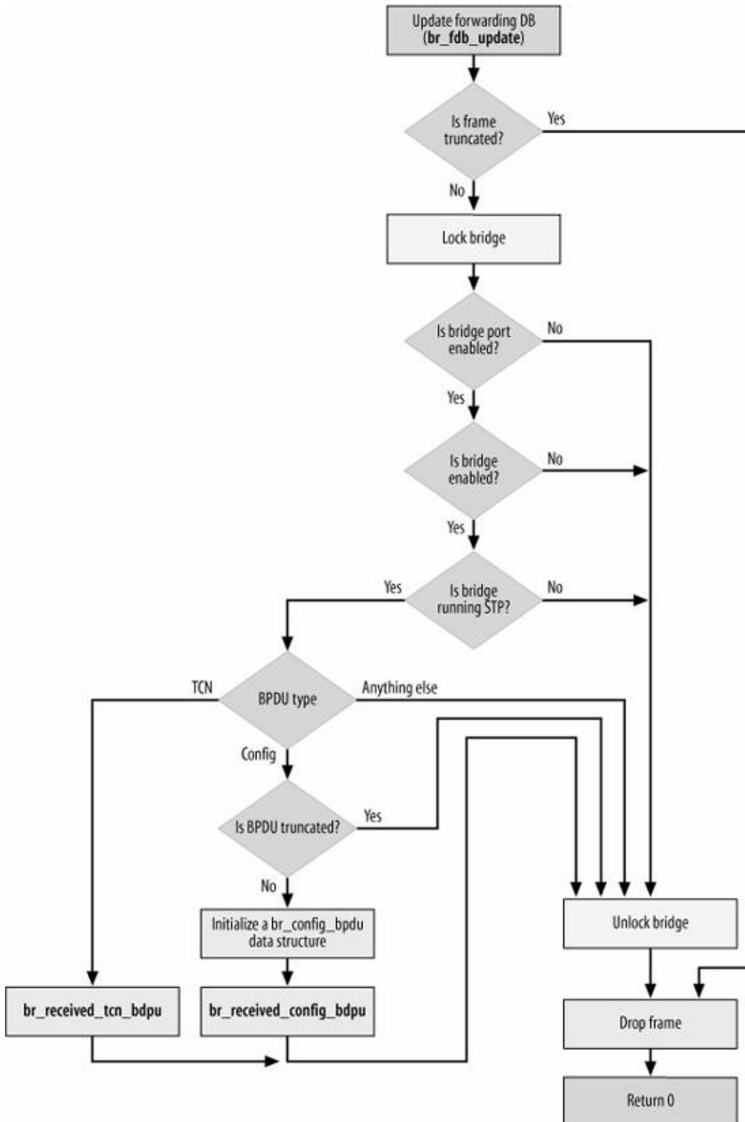
Figure 16-15. br_stp_handle_bpdu function
