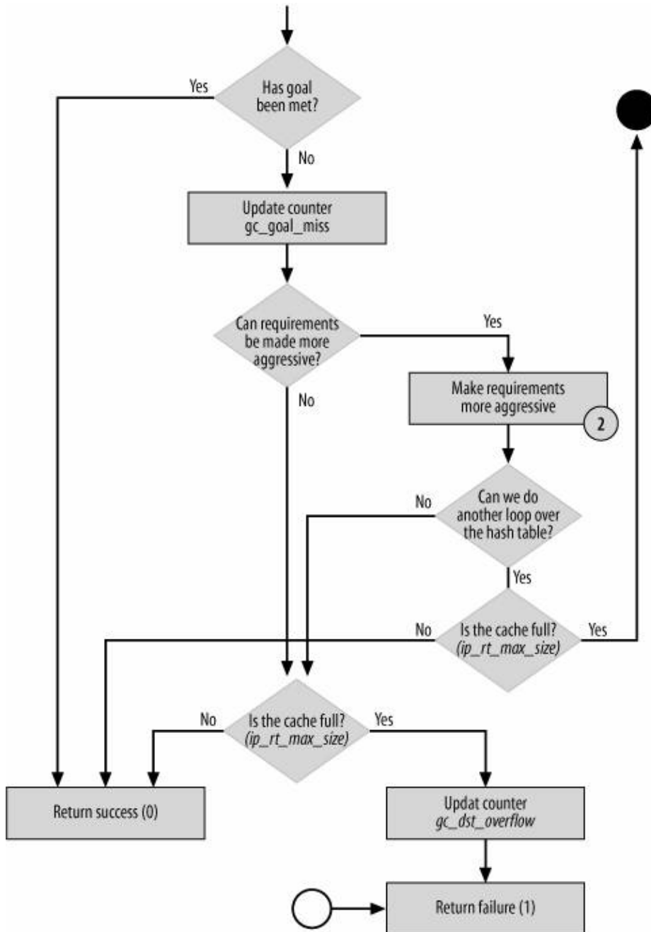
Figure 33-8b. rt_garbage_collect function
