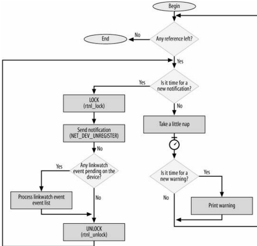
Figure 8-6. Function netdev_wait_allrefs
