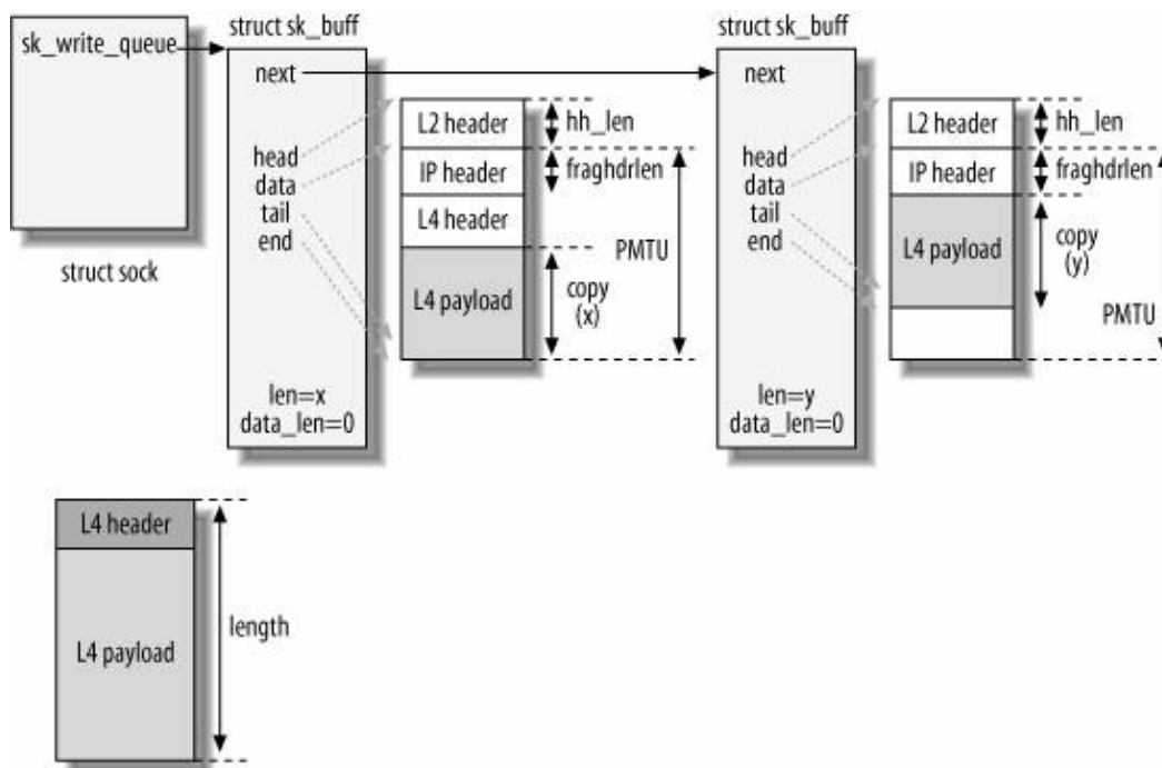
Figure 21-4. Fragmentation without Scatter/Gather I/O, MSG_MORE
