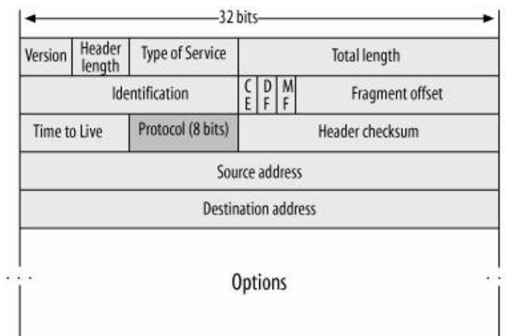
Figure 24-3. IPv4 header and protocol identifier field
