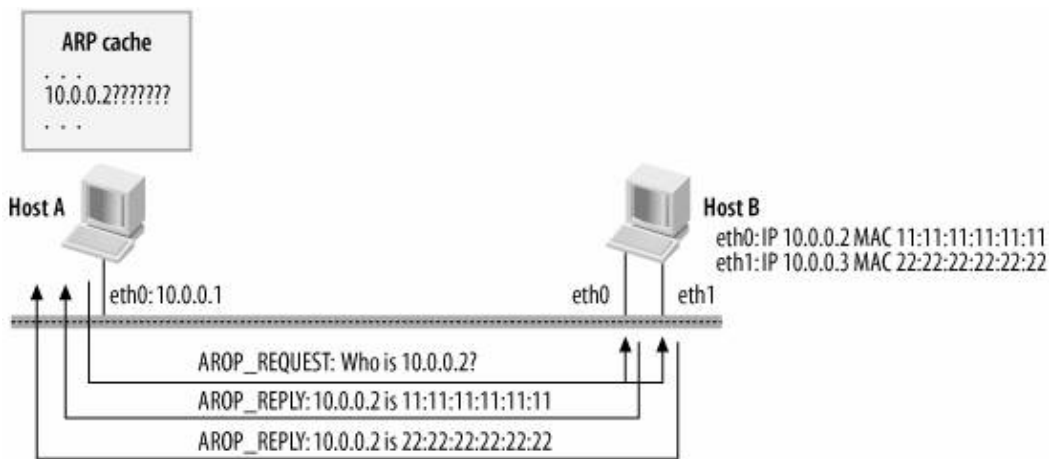
Figure 28-5. The ARP flux problem
