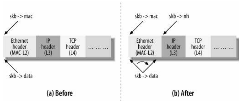
Figure 2-3. Header's pointer initializations while moving from layer two to layer three
