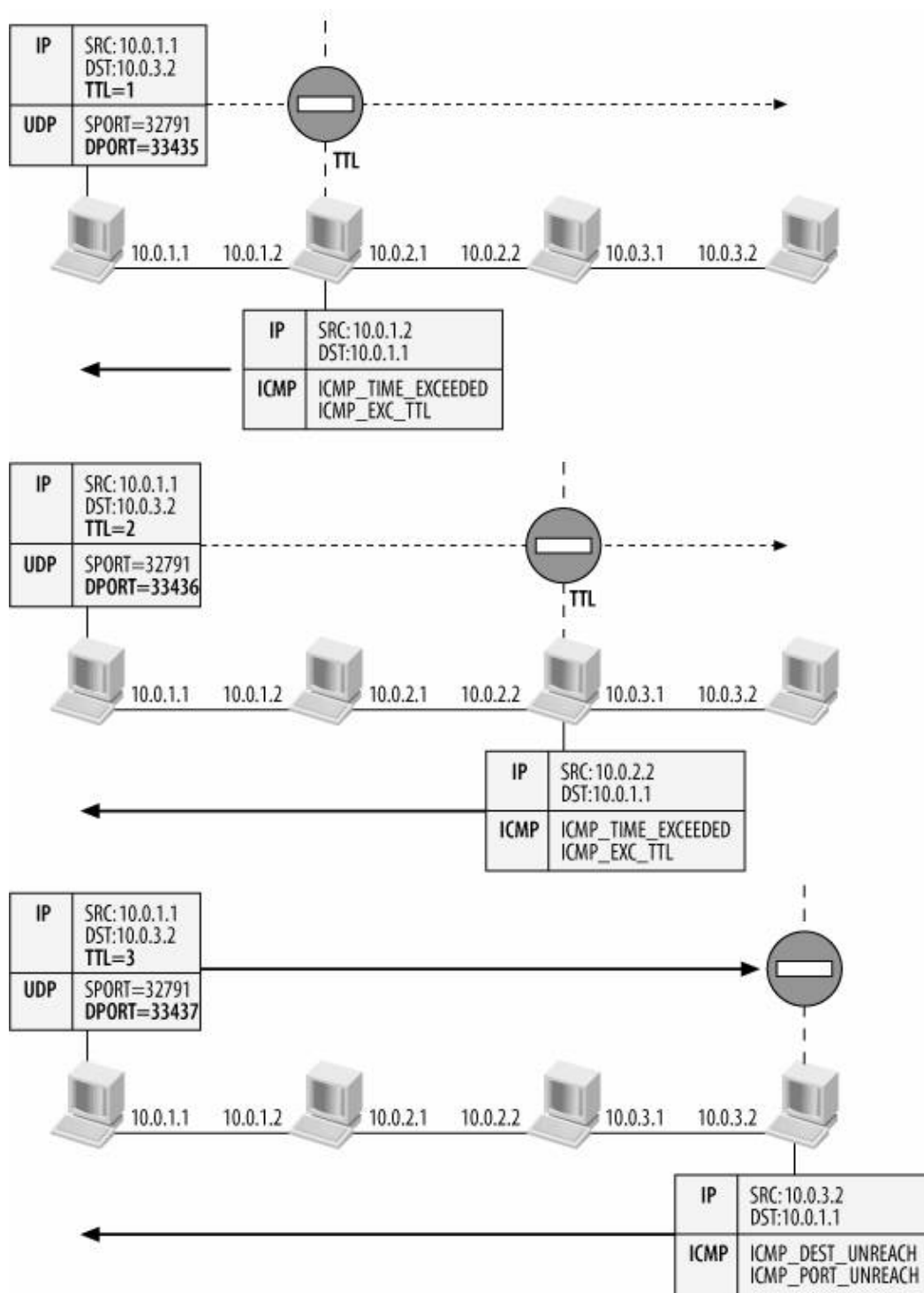
Figure 25-6. Example of traceroute with UDP
