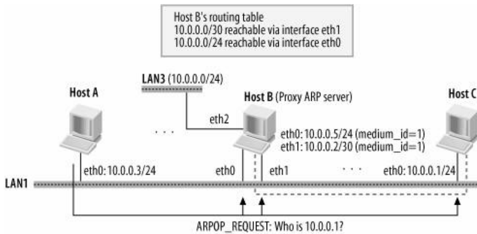
Figure 28-8. Example of use of medium ID
