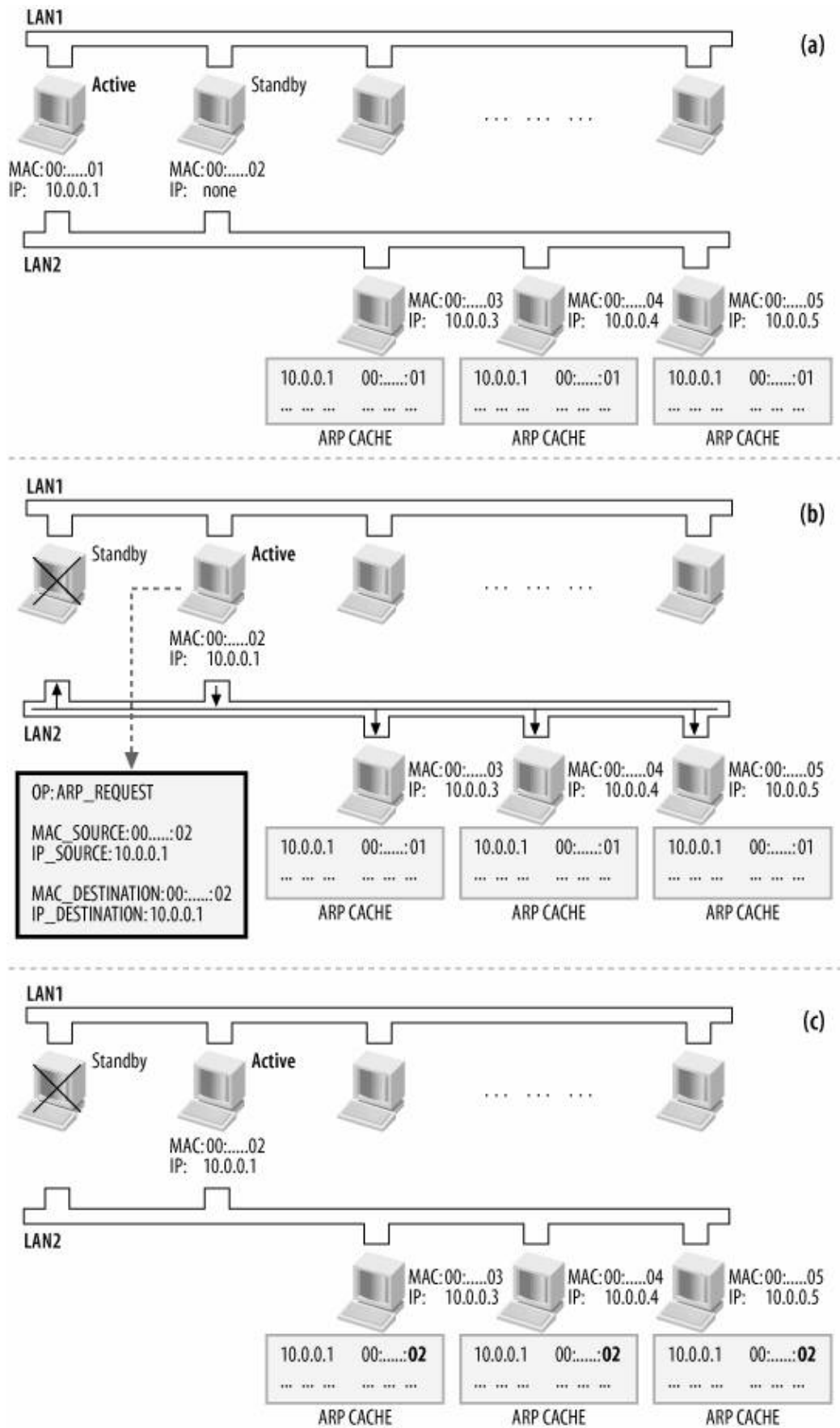
Figure 28-4. Example of gratuitous ARP
