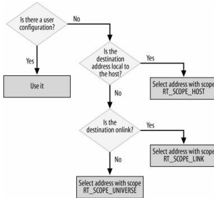
Figure 35-9. Source IP selection
