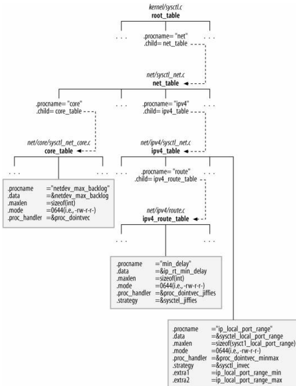
Figure 3-3. Creation of the core directories in /proc/sys/net
