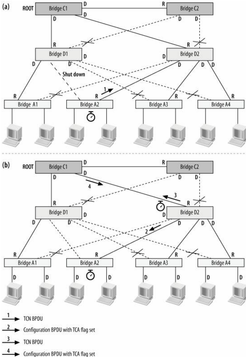
Figure 15-18. Use of the TCN BPDU
