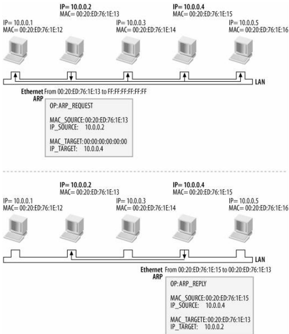
Figure 28-2. Example of ARP usage
