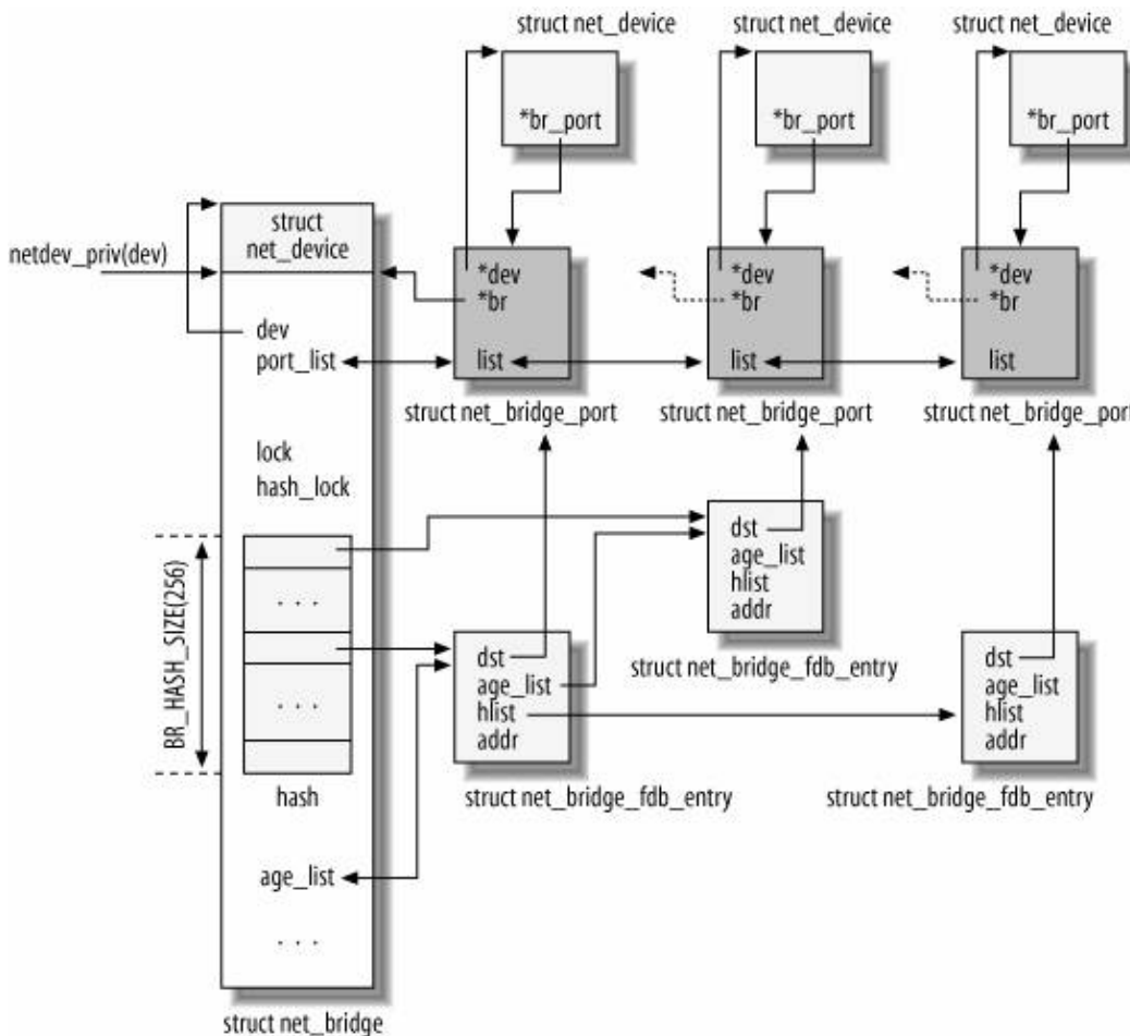
Figure 16-6. Relationships between the main data structure types
