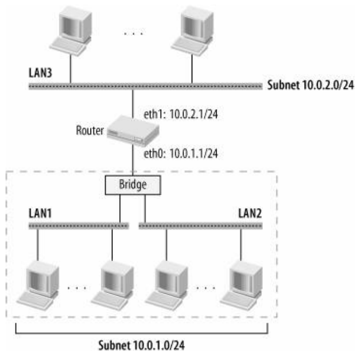
Figure 16-1. Example of use of a bridge
