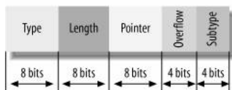
Figure 18-8. IP Timestamp option header
