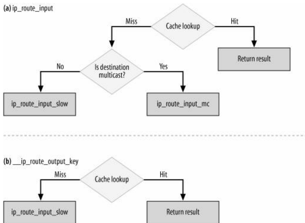
Figure 33-3. (a) ip_route_input_key function; (b) _ _ip_route_output_key function
