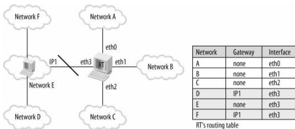
Figure 4-1. Example of Linux router
