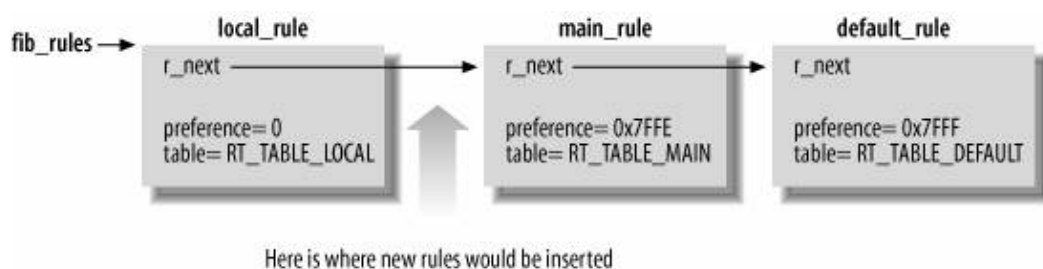
Figure 35-11. Default rules
