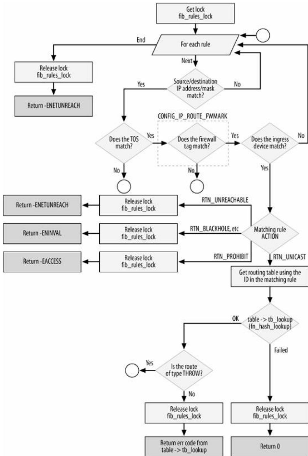
Figure 35-12. Policy Routing version of fib_lookup function
