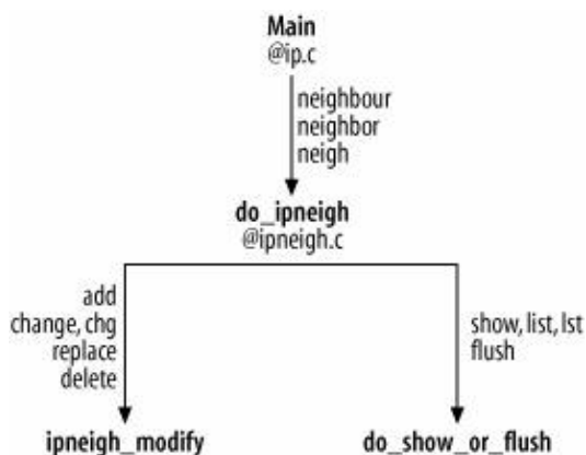
Figure 29-2. Structure of IPRROUTE2 package's neighbor files and functions
