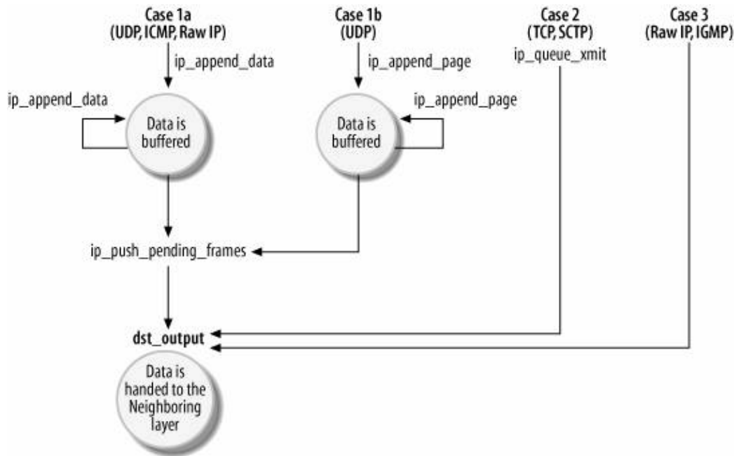
Figure 21-1. Different protocols invoking dst_output differently
