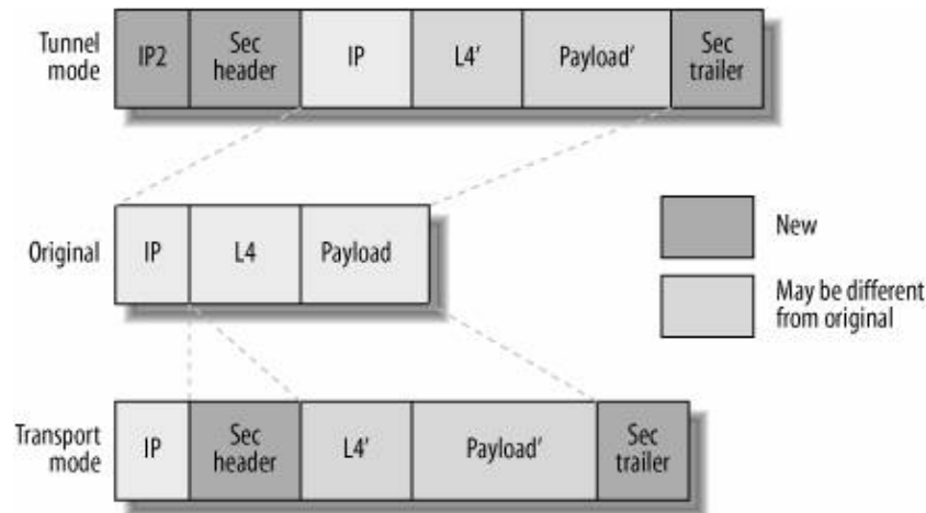
Figure 24-5. IPsec headers/trailers locations
