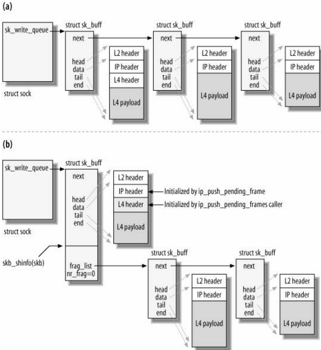
Figure 21-12. (a) Before and (b) after removing buffers from the sk_write_queue queue
