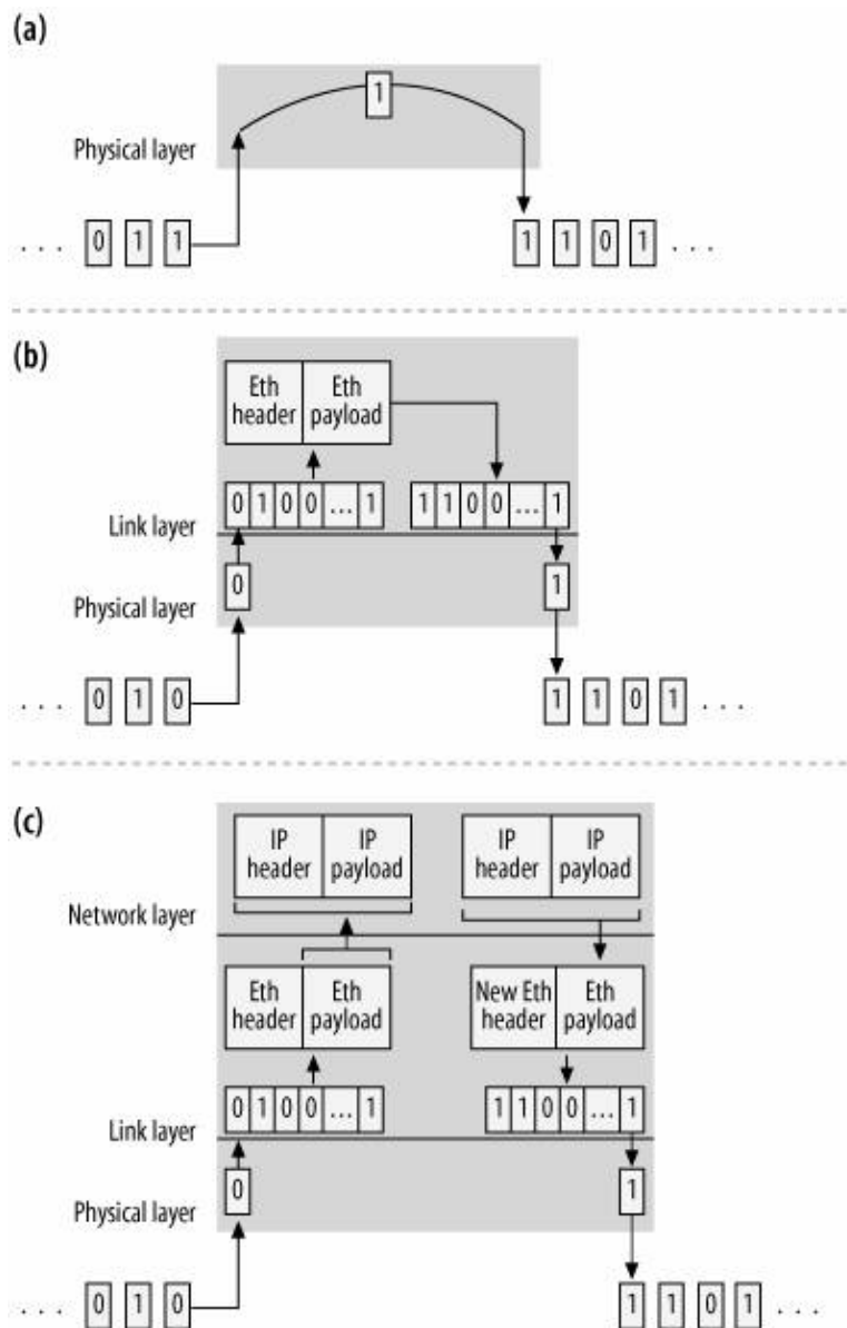
Figure 14-1. (a) Repeater; (b) bridge; (c) router
