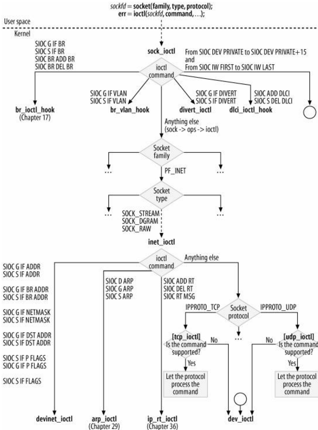
Figure 3-4. Dispatching ioctl commands
