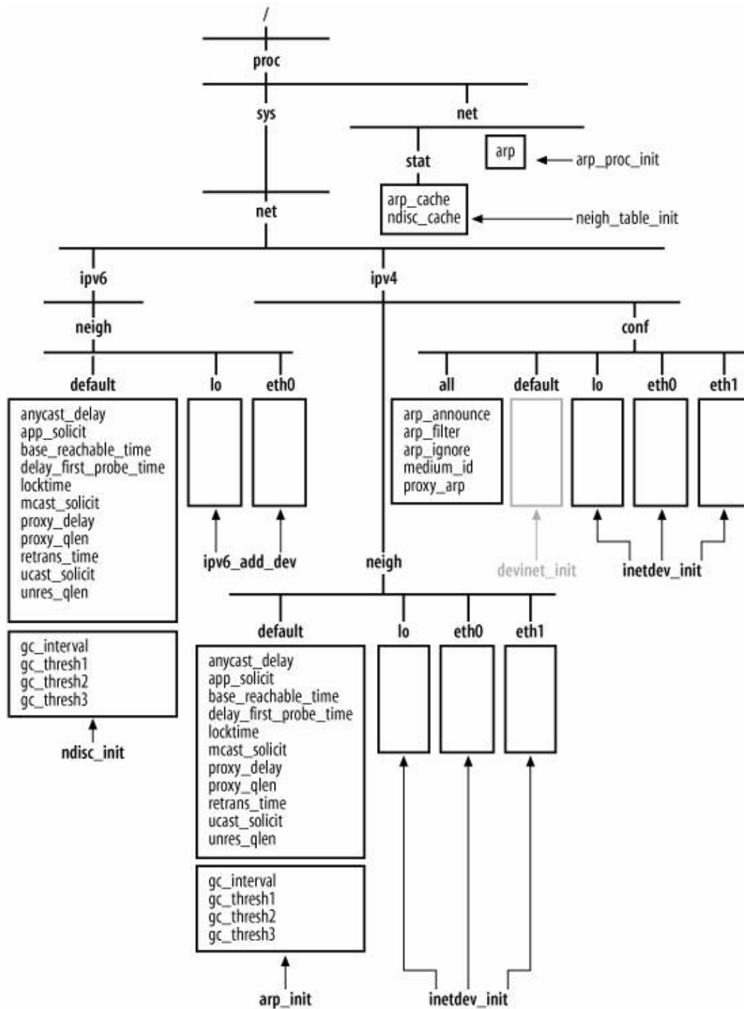
Figure 29-3. Example of /proc/sys file registration for the neighboring subsystem
