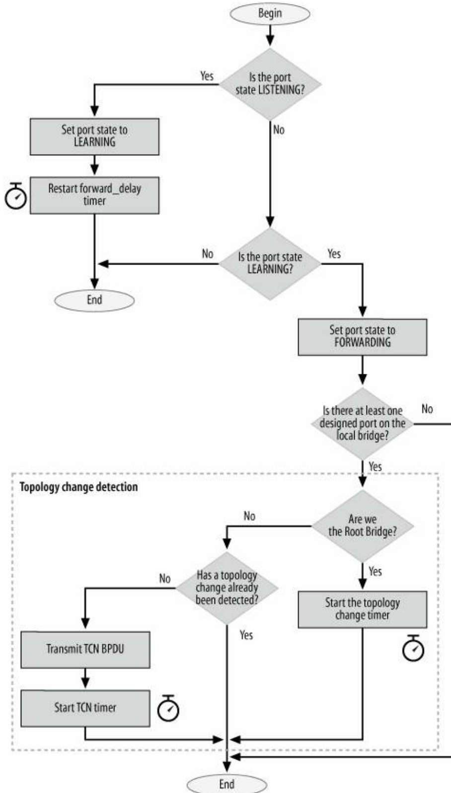
Figure 15-15. Handling the Forward Delay timer
