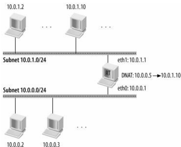
Figure 28-19. DNAT example
