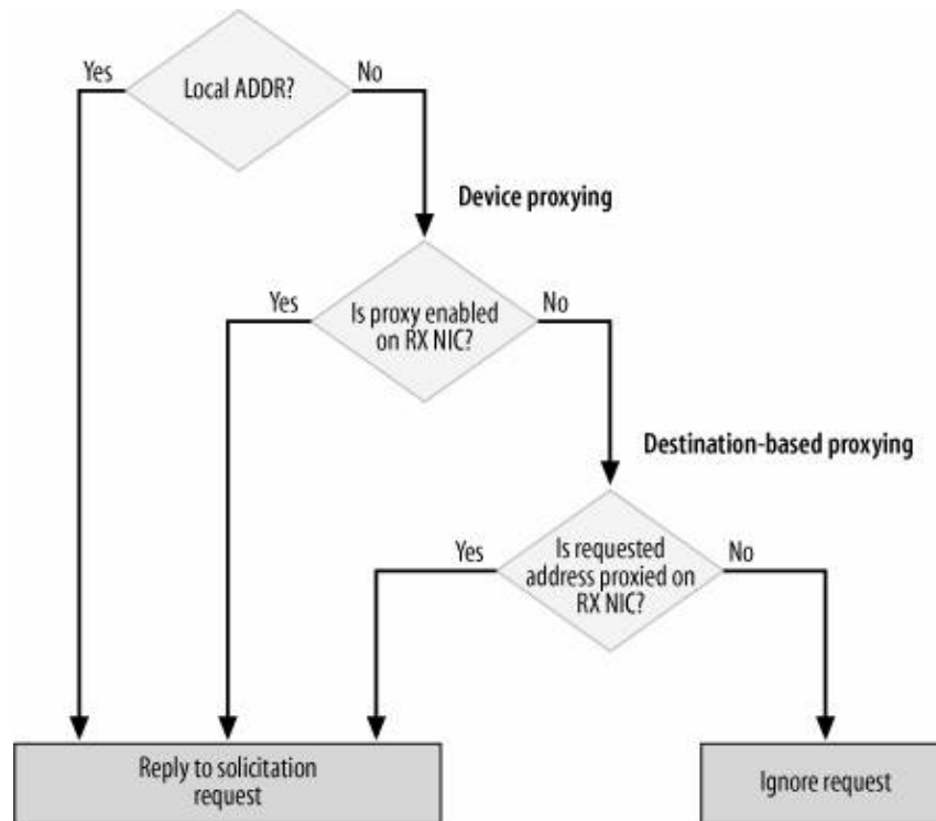
Figure 26-8. Priority between device and address proxying
