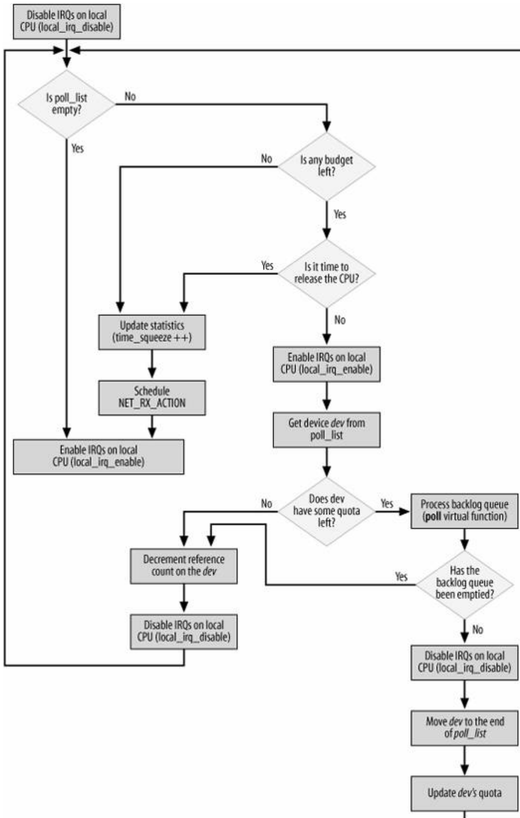
Figure 10-5. net_rx_action function
