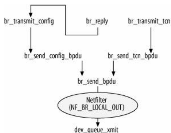
Figure 16-16. Transmit routines
