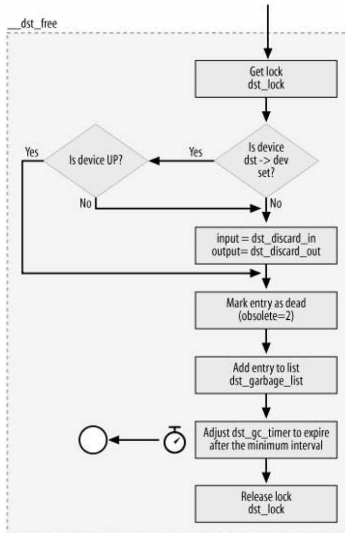
Figure 33-10b. dst_free function
