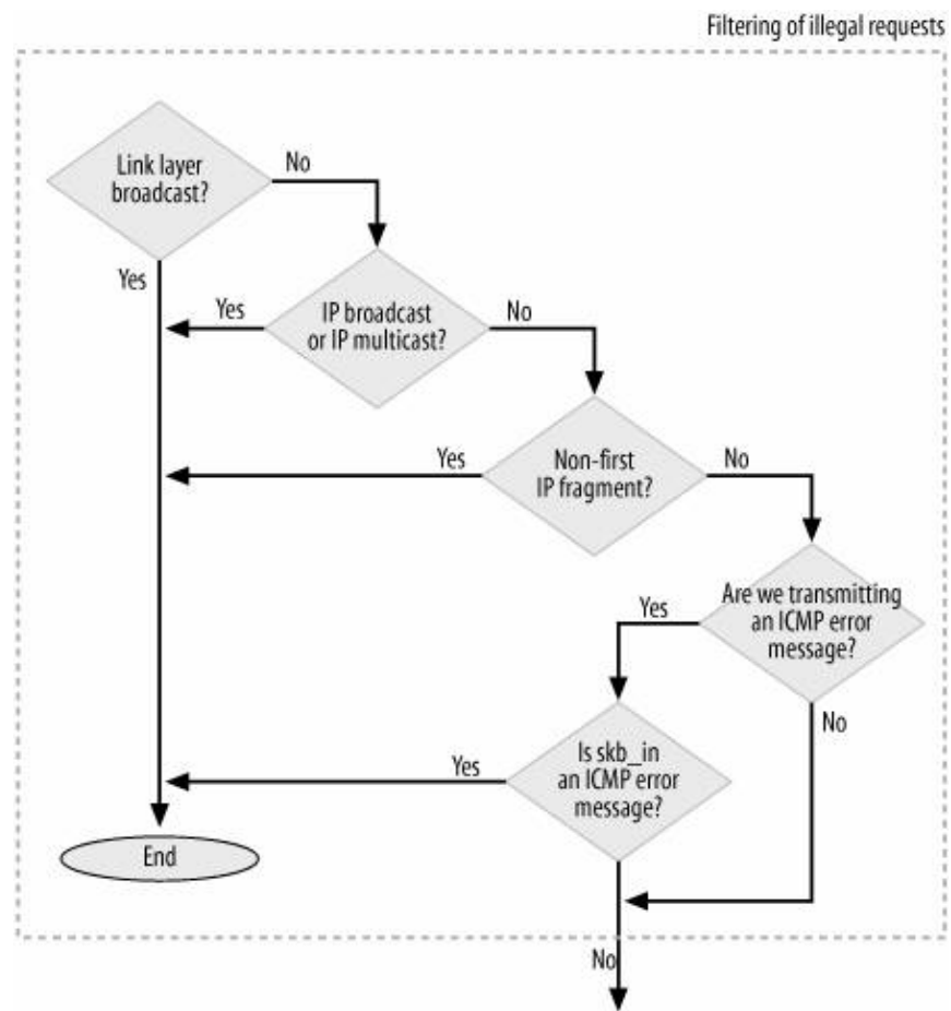
Figure 25-9b. icmp_send function
