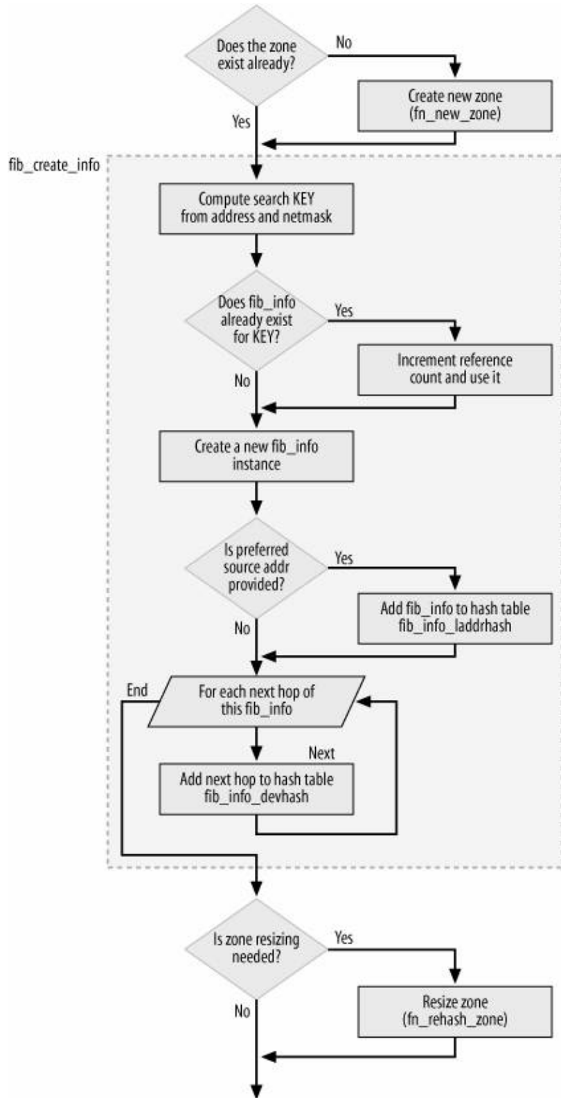
Figure 34-3b. fn_hash_insert function
