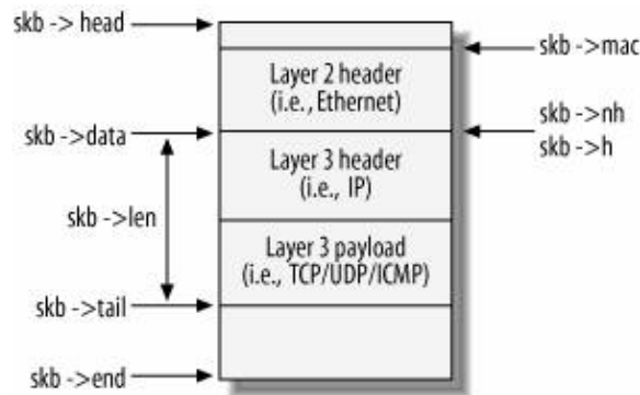
Figure 19-1. Part of sk_buff data structure at the beginning of ip_rcv
