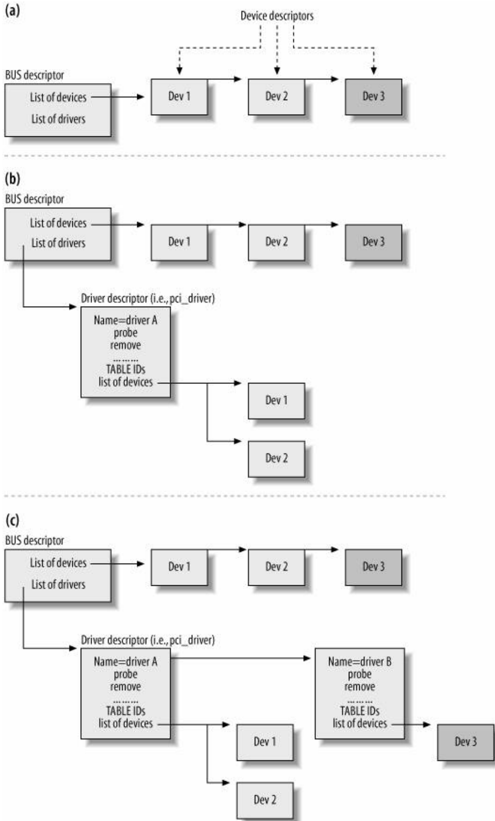
Figure 6-1. Binding between bus and drivers, and between driver and devices
