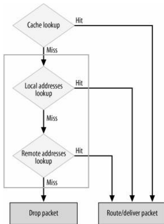
Figure 30-8. Routing lookup
