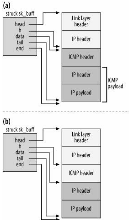
Figure 25-12. (a) skb at the beginning of icmp_rcv ; (b) skb as it is passed to the handler
