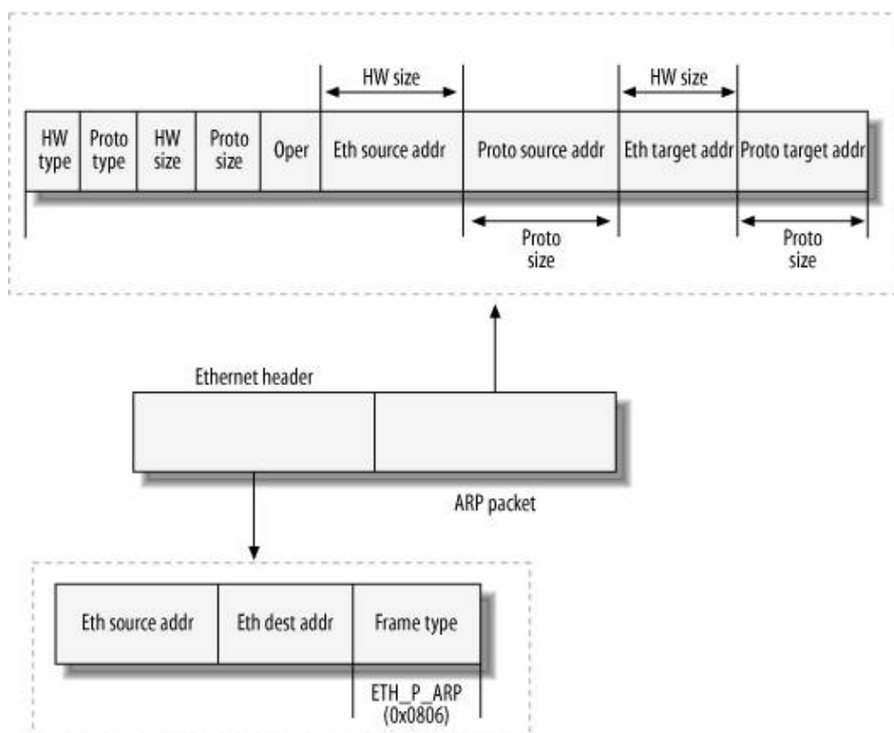
Figure 28-1. ARP packet encapsulated in an Ethernet frame
