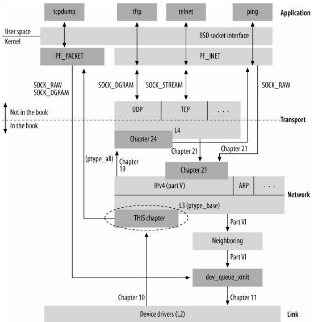
Figure 13-2. The big picture
