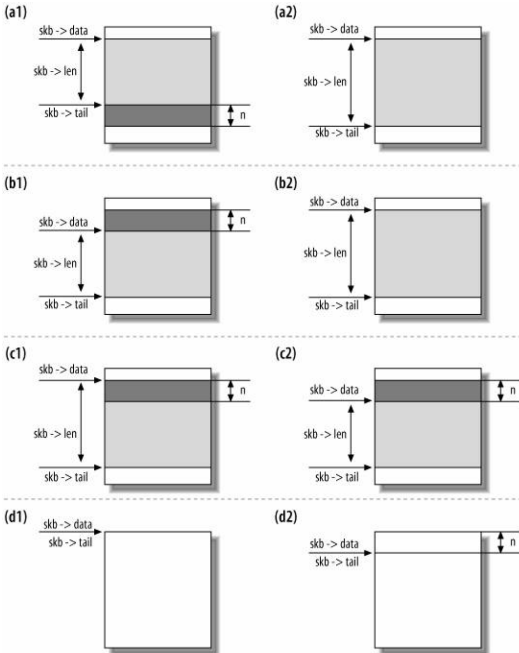
Figure 2-4. Before and after: (a)skb_put, (b)skb_push, (c)skb_pull, and (d)skb_reserve
