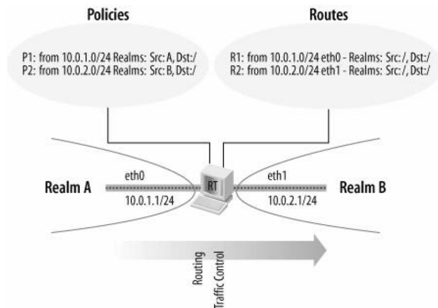
Figure 31-7. Example of realm configuration
