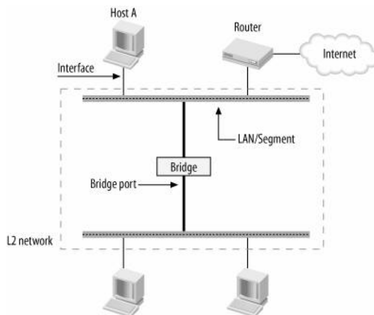
Figure 15-1. Basic terminology
