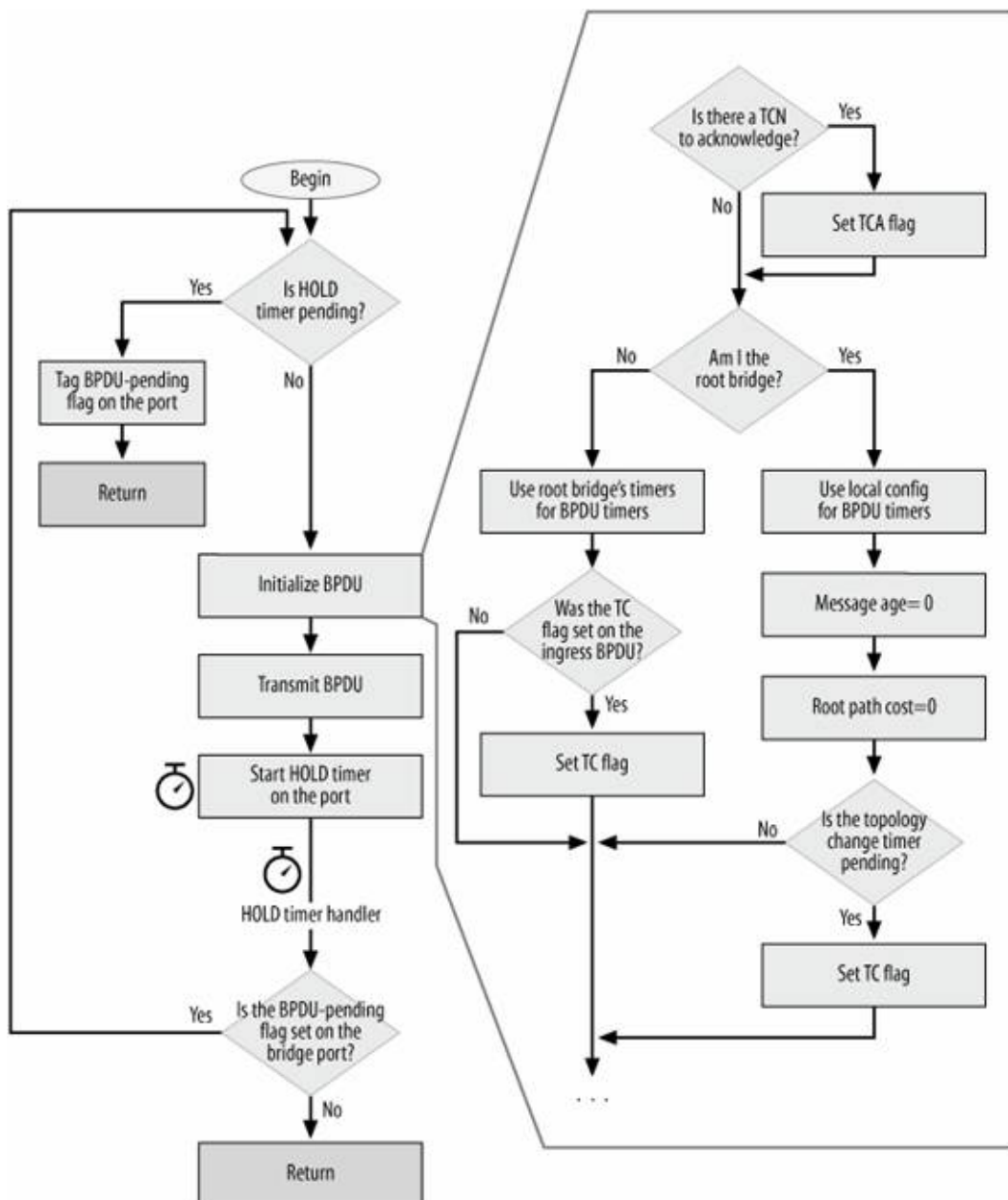
Figure 15-21. Configuration BPDU transmission logic
