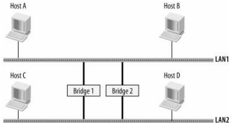
Figure 14-7. Redundant bridges
