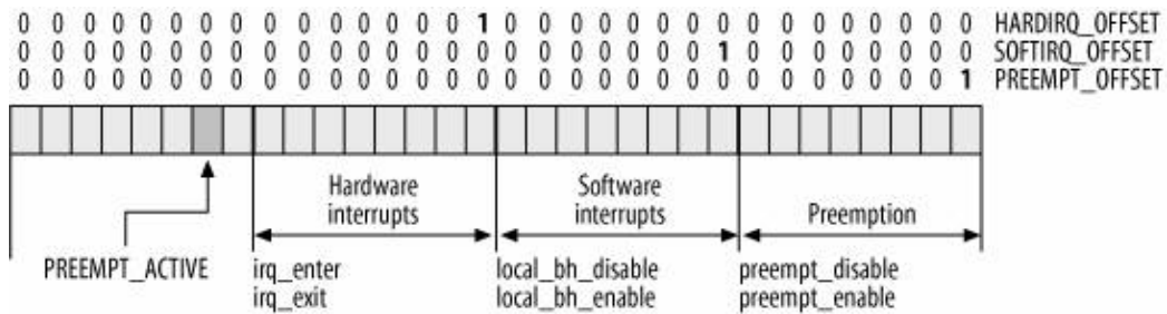
Figure 9-3. Structure of preempt_count
