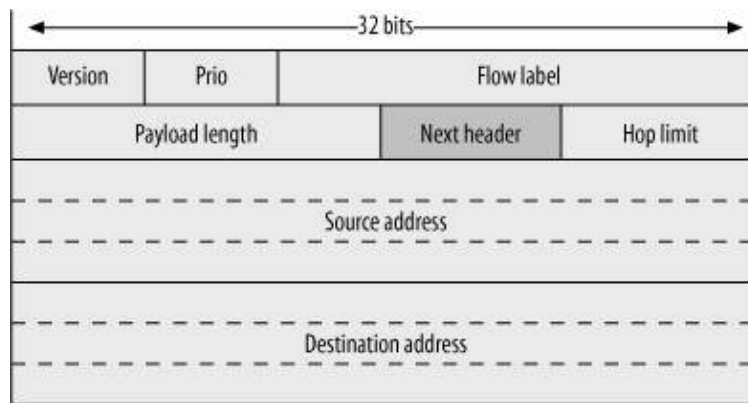
Figure 24-8. IPv6 header and next_header protocol identifier
