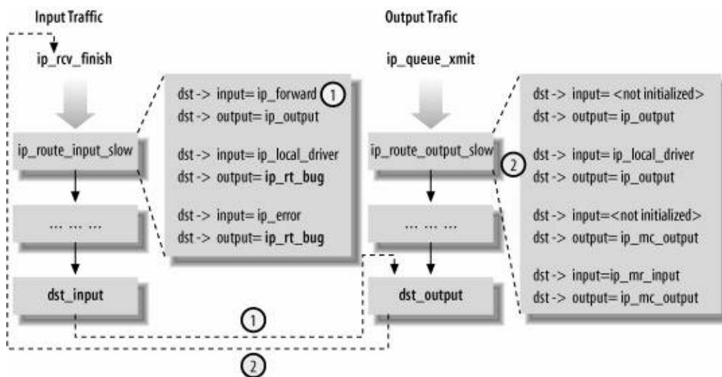
Figure 35-3. dst->input and dst->output initialization
